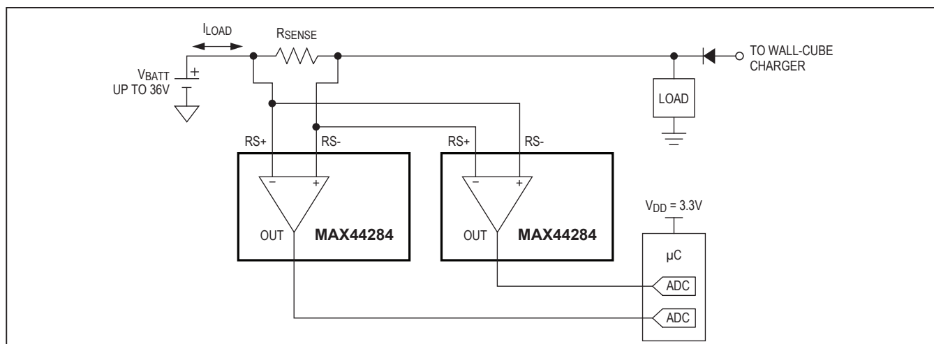
Figure 4. Bidirectional Application
