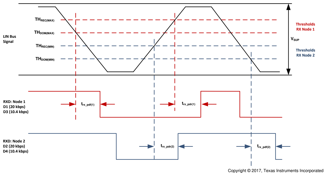
Figure 8-14. Propagation Delay
