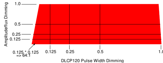
Figure 7-6. Continuous Mode Dimming Illustration 2
