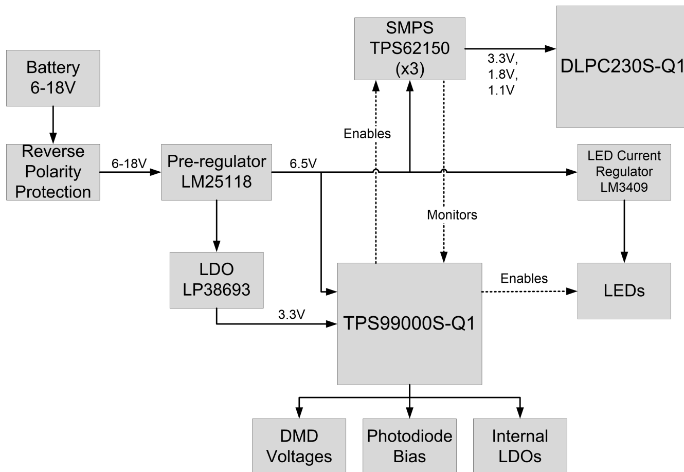
Figure 9-1. Architecture Number 1: HUD Application with LED Forward Voltage Less Than 5 V
