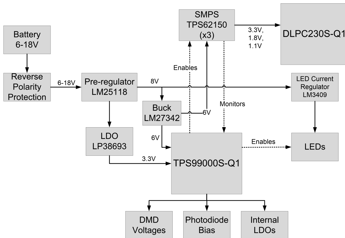
Figure 9-2. Architecture Number 2: HUD Application with Two LEDs in Series Configuration
