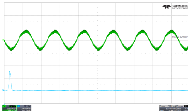
Figure 8-7. Phase current and FFT - Dead time compensation enabled
