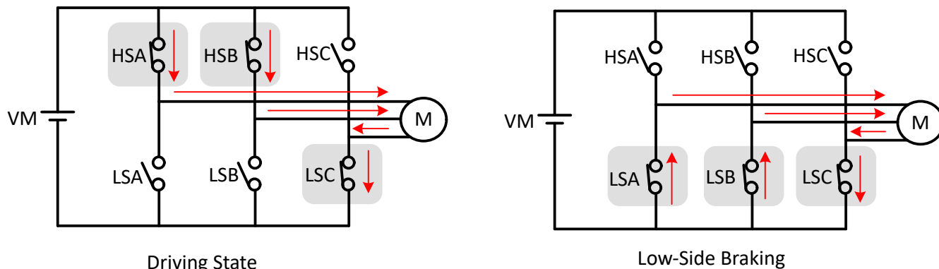
Figure 7-47. Low-Side Braking
