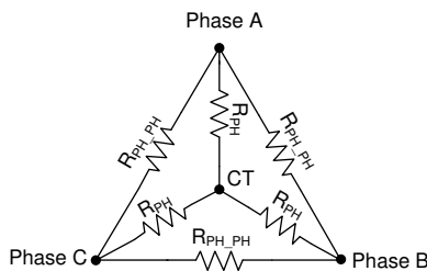
Figure 7-38. Motor Resistance
