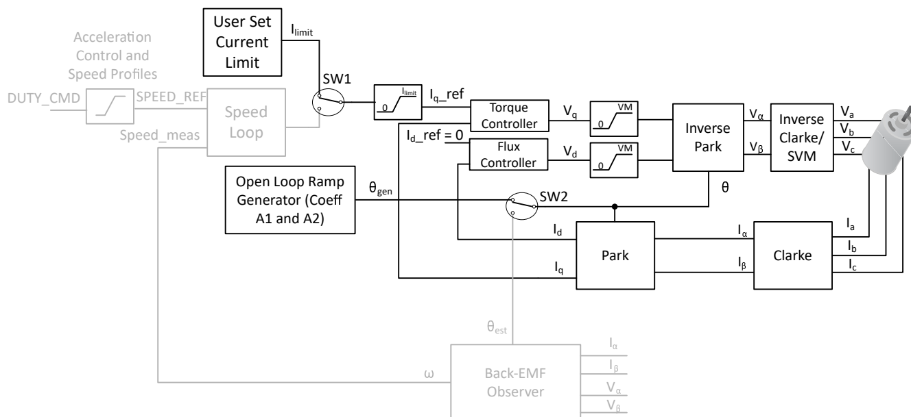
Figure 7-30. Open Loop
