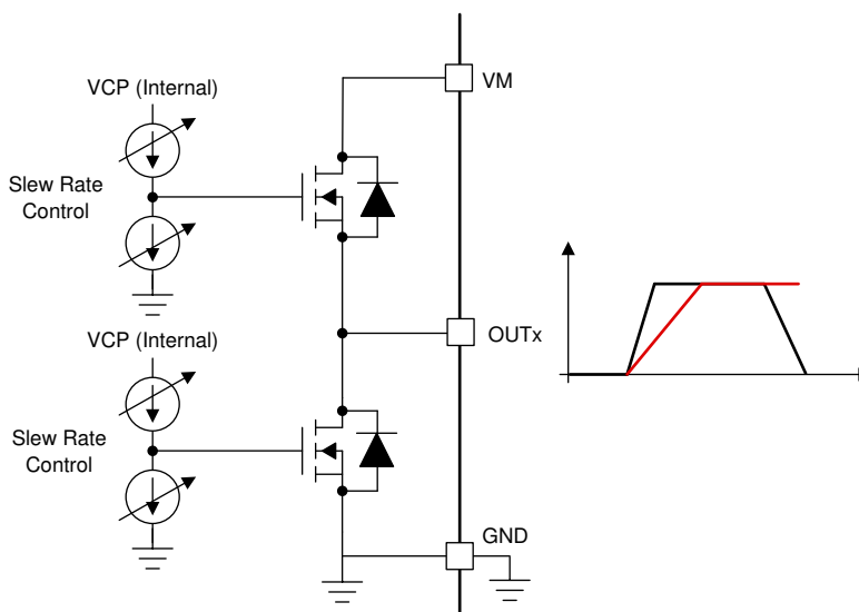
Figure 7-9. Slew Rate Circuit Implementation
