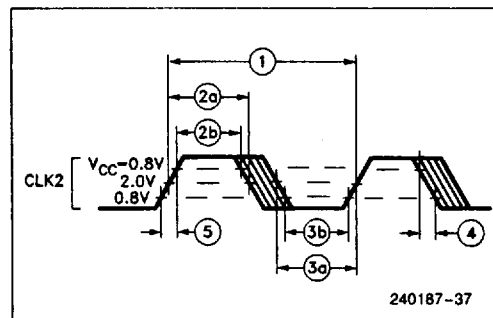
Figure 7.3. CLK2 Waveform
