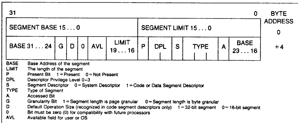
Figure 4.4. Segment Descriptors
