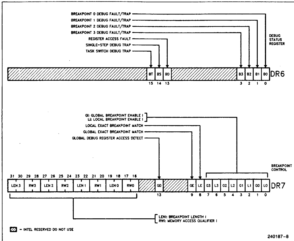
Figure 2.7. Debug Registers
