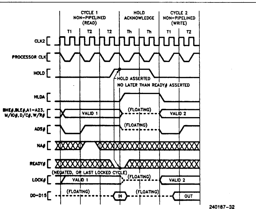
Figure 5.17. Requesting Hold from Active Bus (NA# inactive)
