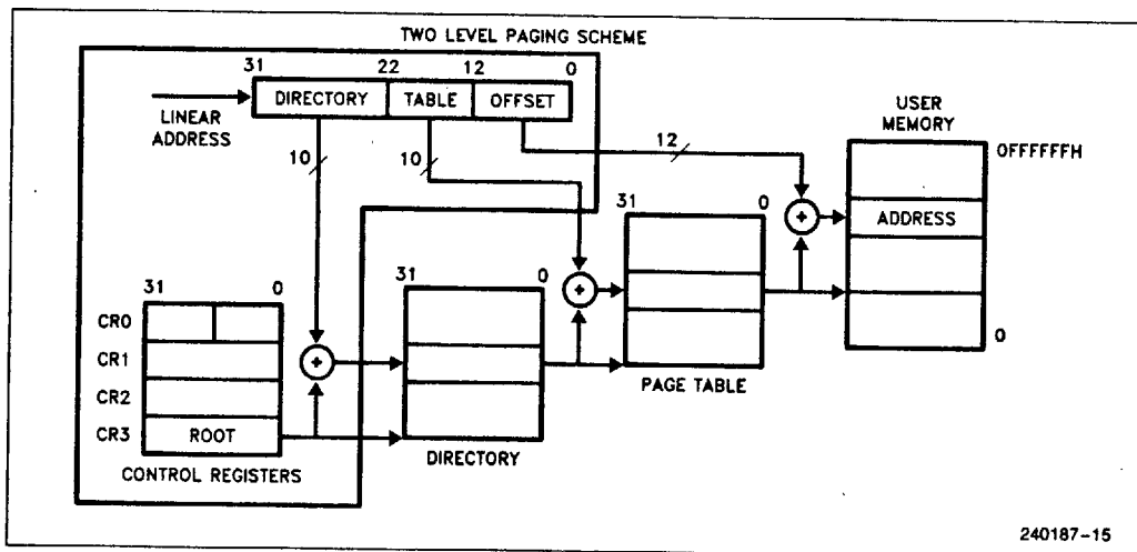
Figure 4.10. Paging Mechanism
