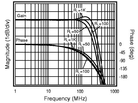
Gain Flatness and Linear Phase
