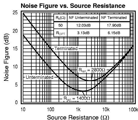
Figure 2: Noise Figure vs. Source Resistance
