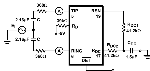
FIGURE 3B. ON-HOOK
