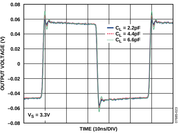
Figure 27. Small Signal Transient Response vs. Capacitive Load
