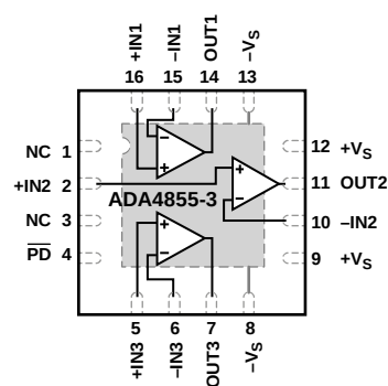
Figure 4. Pin Configuration
