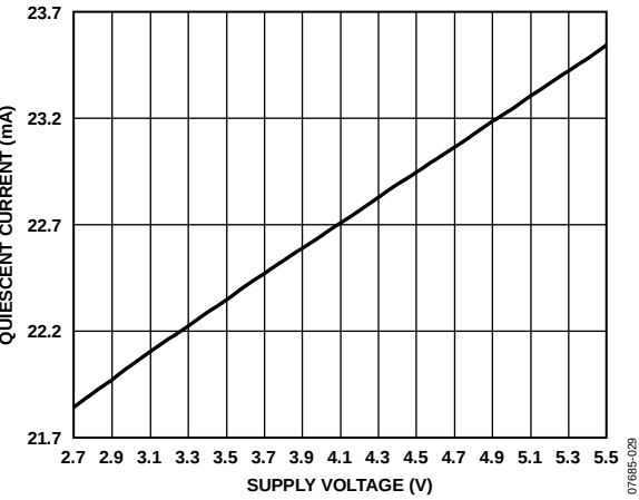
Figure 28. Quiescent Current vs. Supply Voltage
