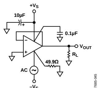
Figure 44. Negative Power Supply Rejection
