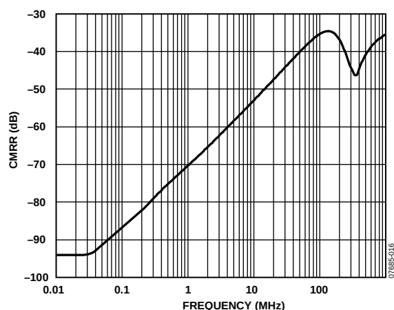
Figure 21. Common-Mode Rejection Ratio (CMRR) vs. Frequency
