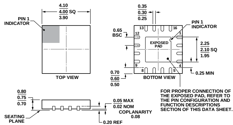
COMPLIANT TO JEDEC STANDARDS MO-220-WGGC. Figure 56.16-Lead Lead Frame Chip Scale Package [LFCSP_WQ] 4 mm × 4 mm Body, Very Very Thin Quad (CP-16-23) Dimensions shown in millimeters
