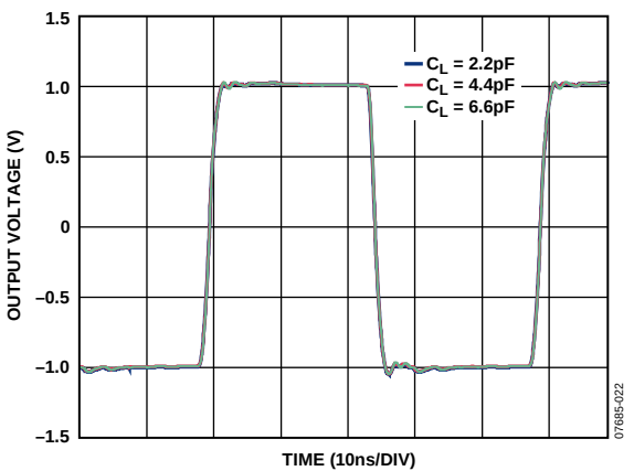
Figure 26. Large Signal Transient Response vs. Capacitive Load
