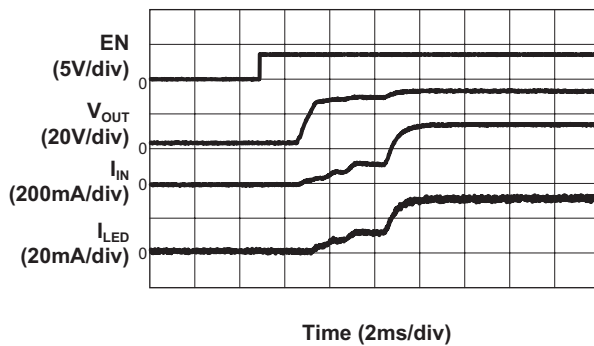
Startup Waveform
