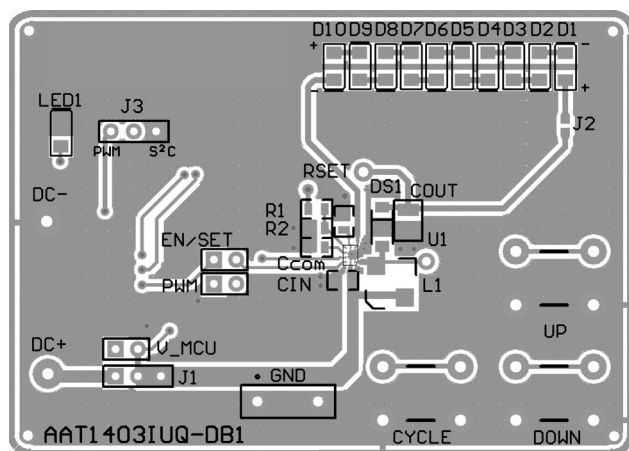
Figure 7: AAT1403 Evaluation Board Top Side Layout.
