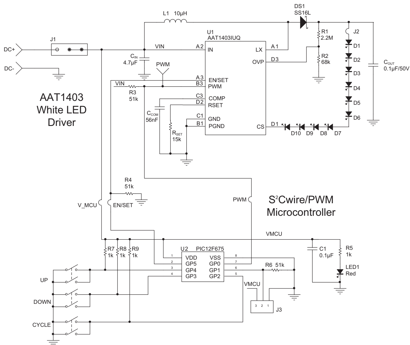
Figure 6: AAT1403 Evaluation Board Schematic.
