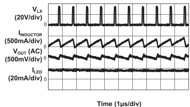
Operation Waveform
