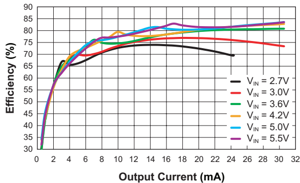
Efficiency vs. Output Current (R SET = 10KΩ, L = 10μH, 10 LEDs)
