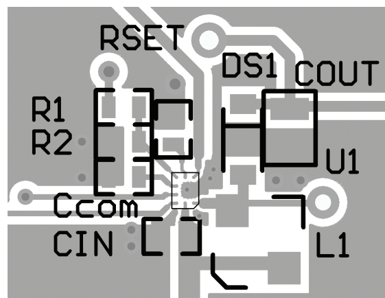
Figure 8: AAT1403 Evaluation Board Top Side Layout (detail).
