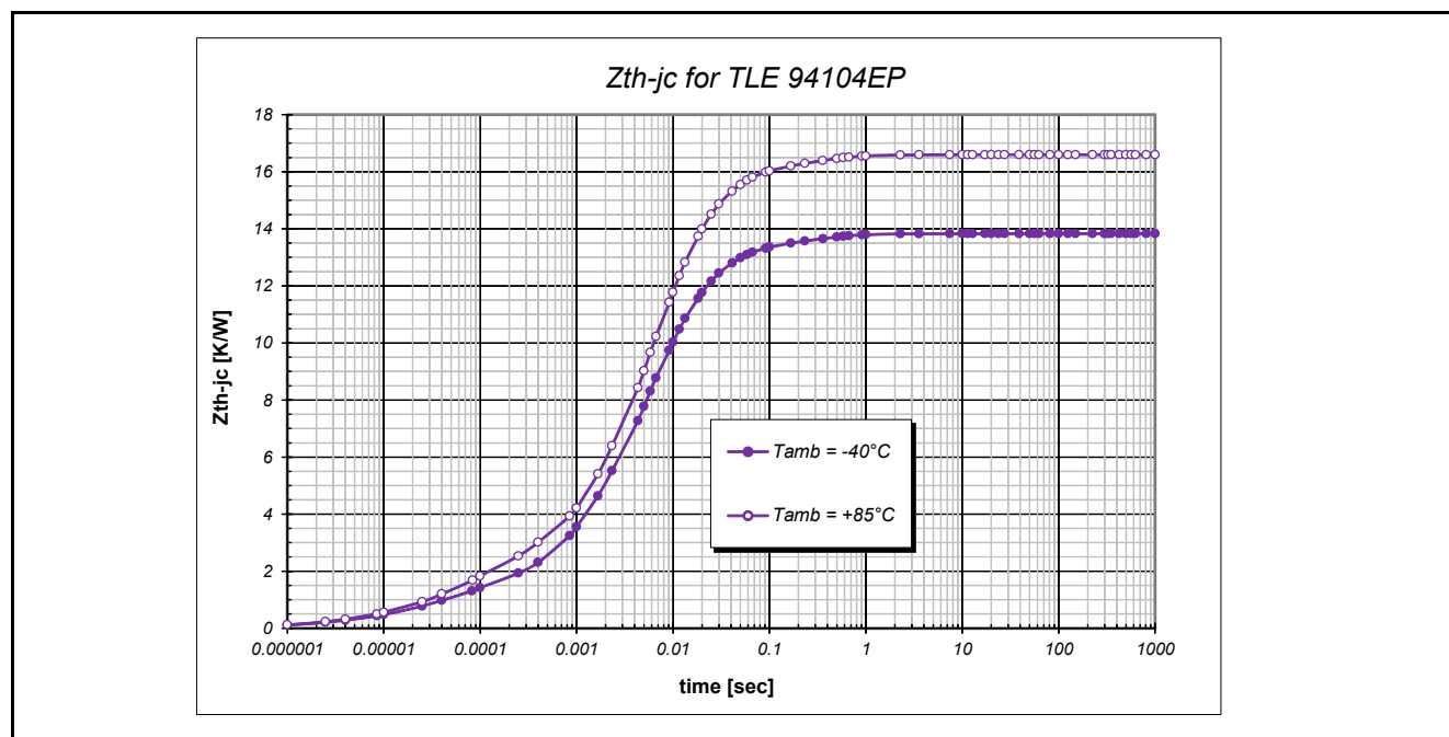
Figure 28 ZthJC Curve
