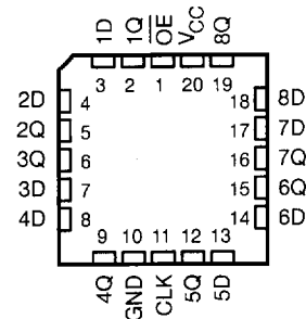
SN54BCT374 . . . FK PACKAGE (TOP VIEW)
