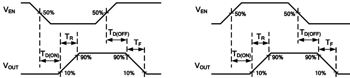
Figure 1. Voltage Waveforms: AP2301A (left), AP2311A (right)
