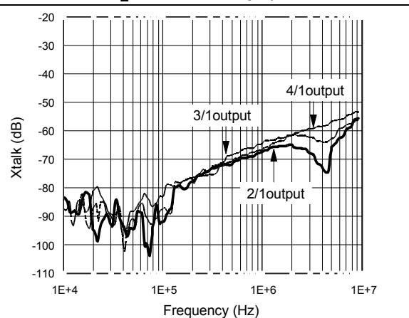
Figure 26. Channel separation (Xtalk) vs. frequency (gain = +11, V_{CC} = \pm 2.5 V, Z_L = 150 \Omega // 27 pF)
