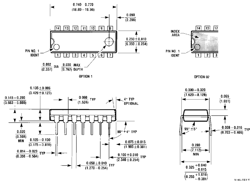
Molded Dual-In-Line Package (N) Order Number DM74ALS21AN Package Number N14A
