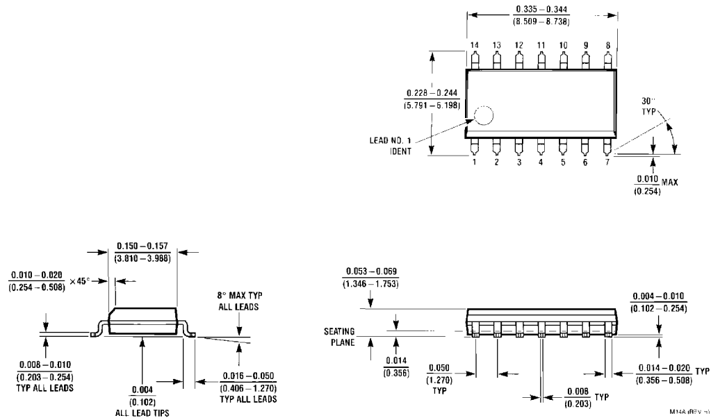
S.O. Package (M) Order Number DM74ALS21AM Package Number M14A
