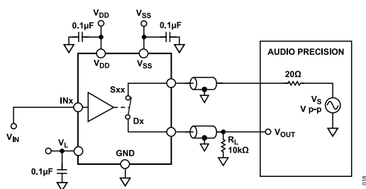
Figure 32. THD + Noise
