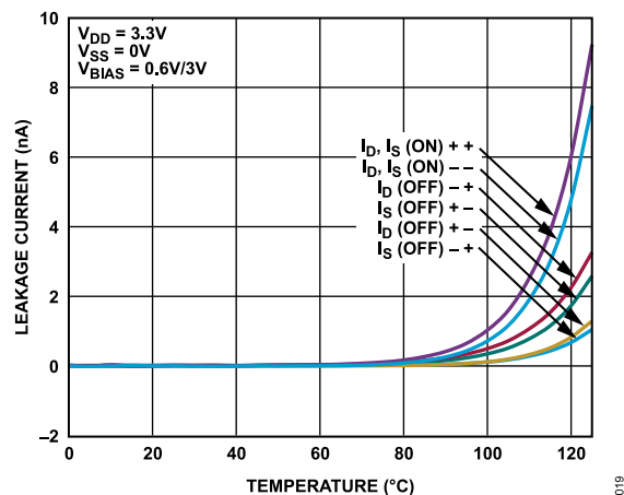
Figure 12. Leakage Current vs. Temperature, 3.3 V Single Supply
