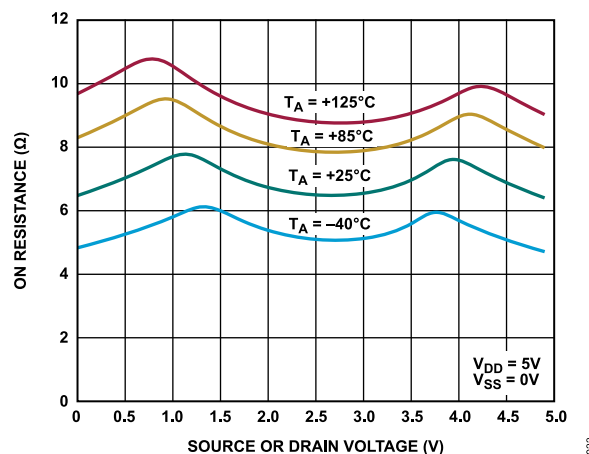
Figure 7. On Resistance vs. V_D ( V_S ) for Different Temperatures, 5 V Single Supply
