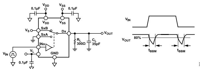
Figure 26. Break-Before-Make Delay, t_{\text{BBM}}
