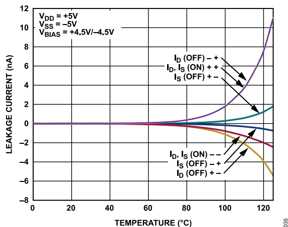
Figure 9. Leakage Current vs. Temperature, \pm 5 V Dual Supply
