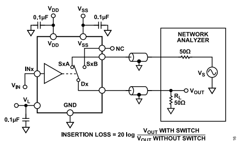
Figure 30. Bandwidth
