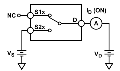
Figure 24. On Leakage
