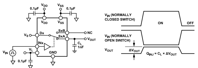
Figure 28. Charge Injection
