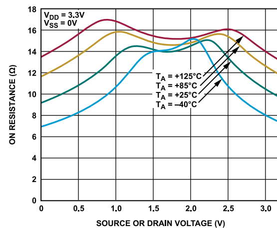
Figure 8. On Resistance vs. V_D ( V_S ) for Different Temperatures, 3.3 V Single Supply
