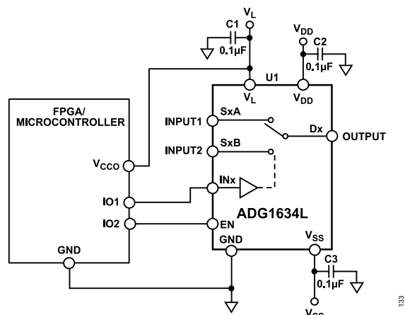
Figure 33. Typical Application
