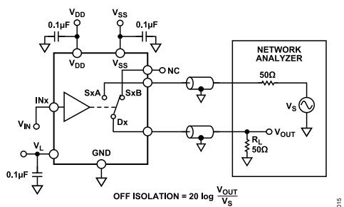
Figure 29. Off Isolation
