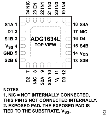
Figure 2. Pin Configuration
