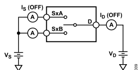
Figure 23. Off Leakage
