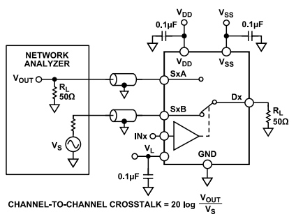
Figure 31. Channel-to-Channel Crosstalk
