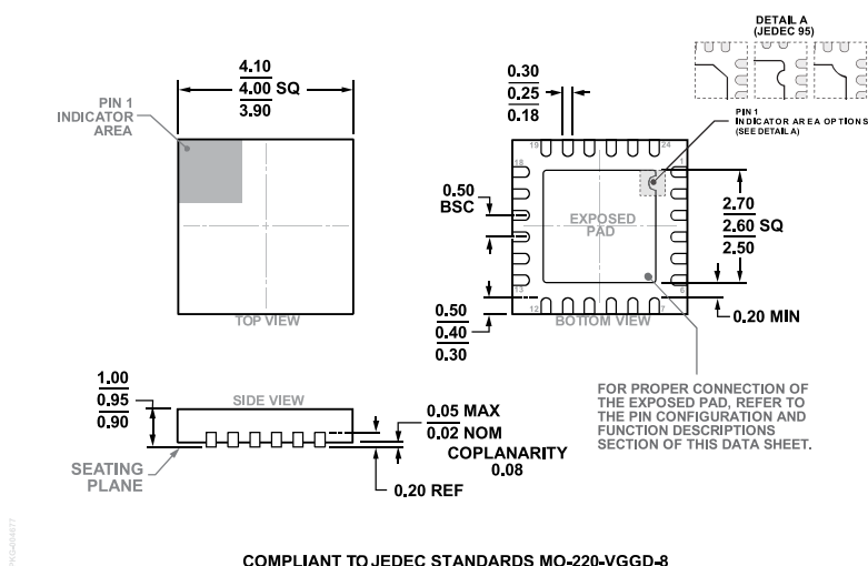
Figure 37. 24-Lead Lead Frame Chip Scale Package [LFCSP] 4 mm × 4 mm Body and 0.95 mm Package Height (CP-24-17) Dimensions shown in millimeters
