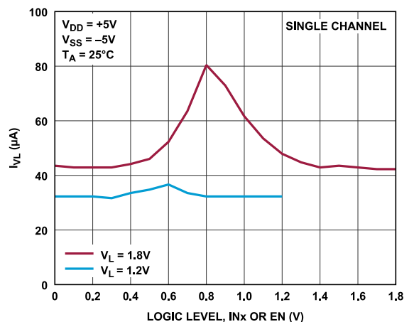
Figure 13. I_{VL} vs. Logic Level, INx or EN
