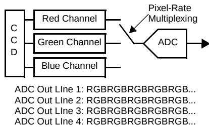
Figure 36: 3 Channel Pixel Rate Mode
