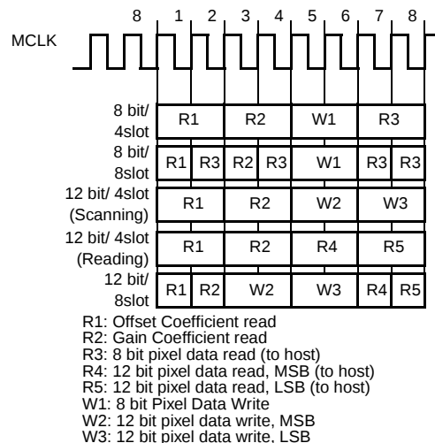
Figure 42: SRAM Access Modes
