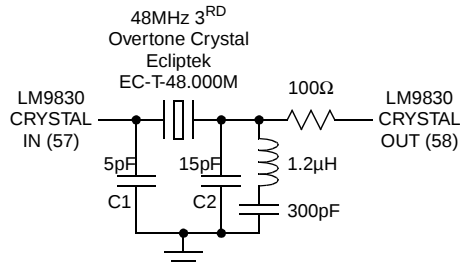
Figure 63: Crystal Oscillator Circuit
