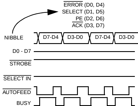
Figure 61: Reading Pixel Data (Nibble Mode)
