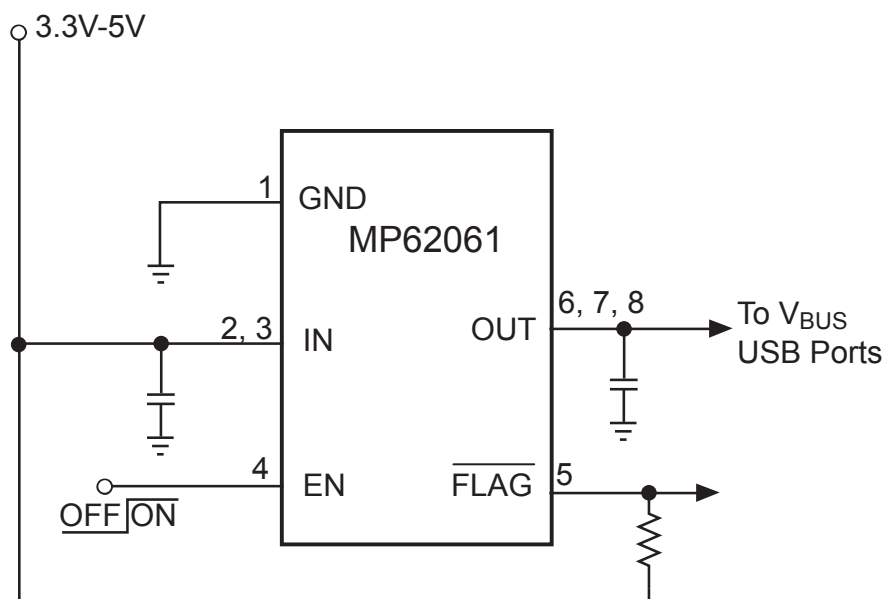
Figure 3—Application Circuit
