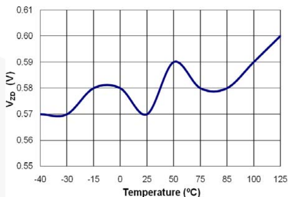
Figure 6. PWM Zero-Duty Voltage ( V_{ZD} ) vs. Temperature
