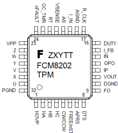
Figure 4. Pin Configuration
