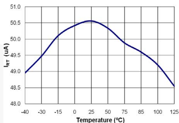
Figure 12. RT Current Source ( I_{RT} ) vs. Temperature
