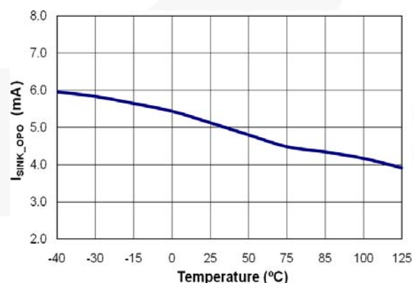
Figure 10. OPO Current Sink ( I_{SINK\_OPO} ) vs. Temperature
