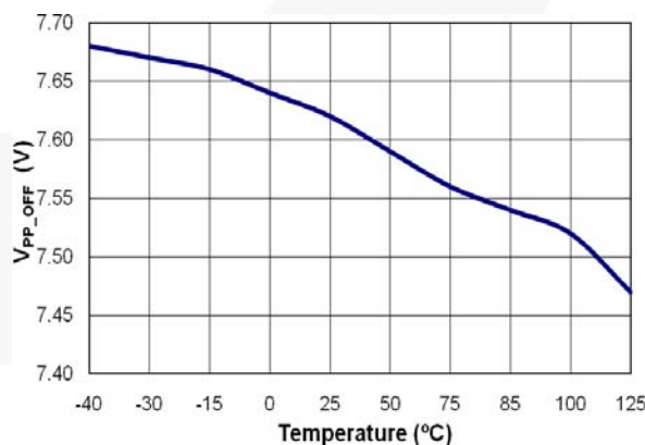
Figure 16. V_{PP} Turn-Off Threshold Voltage ( V_{PP\_OFF} ) vs. Temperature
