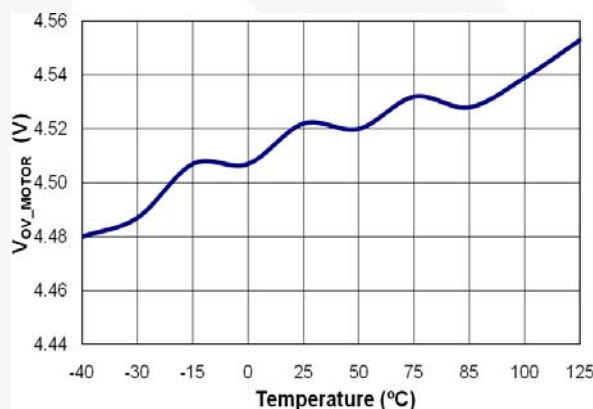
Figure 14. Motor OVP Threshold Voltage ( V_{OV\_MOTOR} ) vs. Temperature
