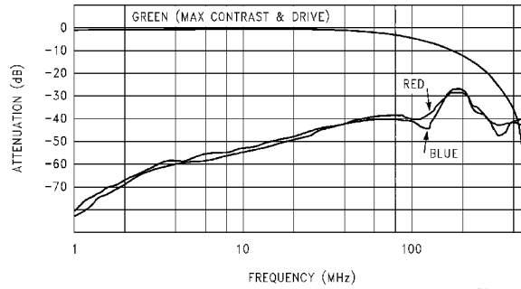
LM1207A Crosstalk vs Frequency
