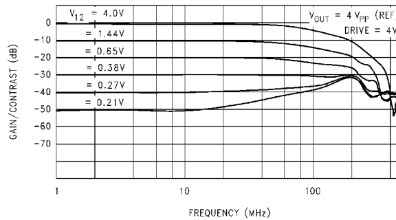
LM1207A Contrast vs Frequency
