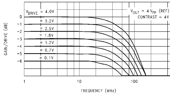
LM1207A Drive vs Frequency
