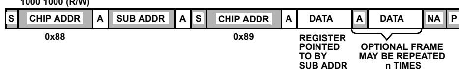
FIGURE 19. REGISTER WRITE/READ FLOW
