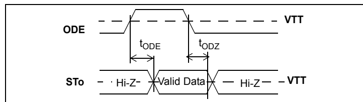
Figure 28 - Output Driver Enable (ODE)
