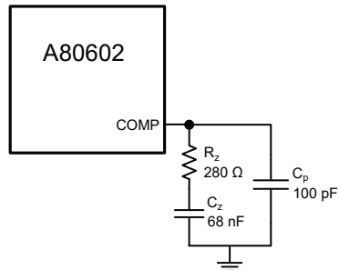
Figure 45: Compensation Network Schematic
