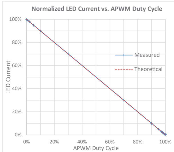
Figure 22: Showing LED current is inversely proportional to the APWM duty cycle. Test conditions: V_{IN} = 12\text{ V} , V_{OUT} = 25\text{ V} ( 8 \times \text{WLED} ), total LED current = 100\text{ mA} \times 4 , APWM frequency = 100\text{ kHz}
