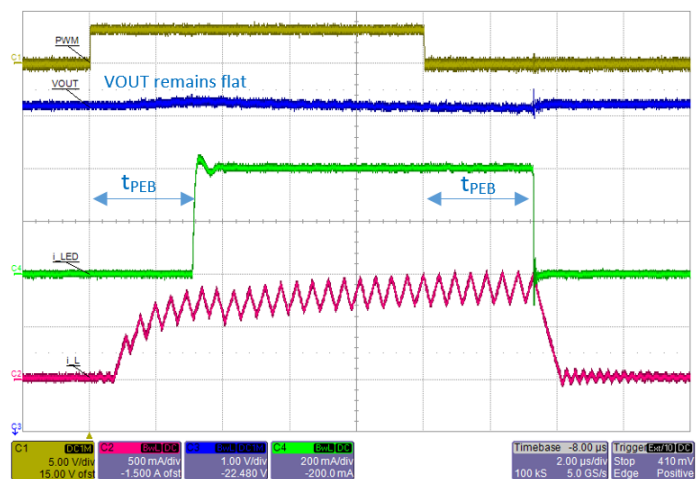
Figure 19: A80602 PWM dimming operation with PEB delay set to 3 \mu s. Note that V_{OUT} ripple is reduced to ~0.2 V.
