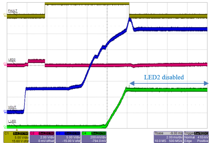
Figure 35: A80602 startup with LED2 string open. V_{OUT} hits OVP at ~30 V and LED2 is removed from regulation. FAULT pin goes Low but remaining LED strings continue to operate.
