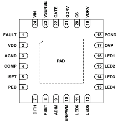
Package ES, 24-Pin QFN Pinouts
