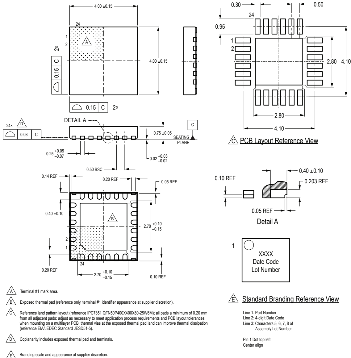
Figure 44: Package ES, 24-Pin 4 mm x 4 mm QFN with Exposed Thermal Pad and Wettable Flank
