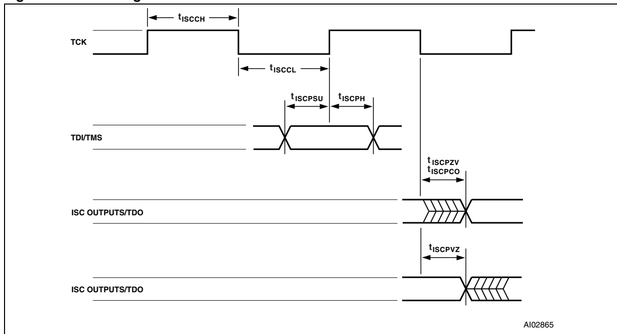
Figure 52. ISC Timing
