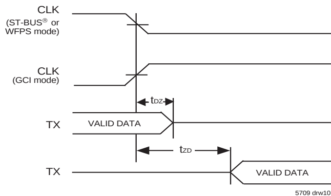
Figure 10. Serial Output
