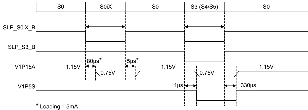
Figure 5. S0iX, S3 (S4/S5) Enter/Exit Sequence
