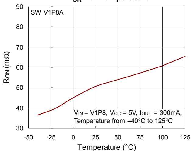
R ON vs. Temperature
