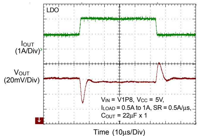
V1P15A Load Transient Response
