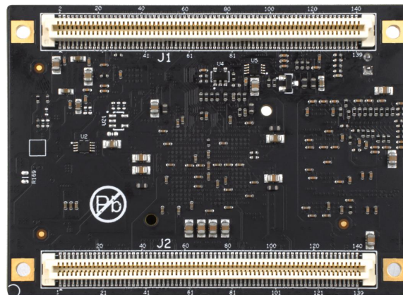
MYC-C7Z010/20-V2 CPU Module Bottom-view
