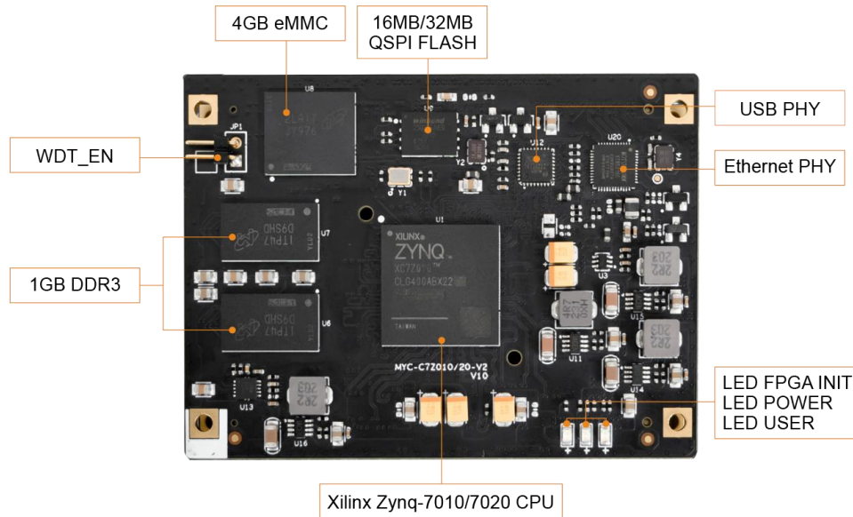
MYC-C7Z010/20-V2 CPU Module Top-view
