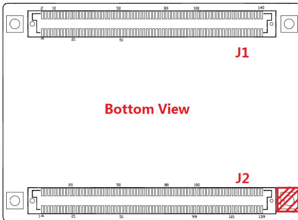
Expansion Connectors of MYC-C7Z010/20-V2
