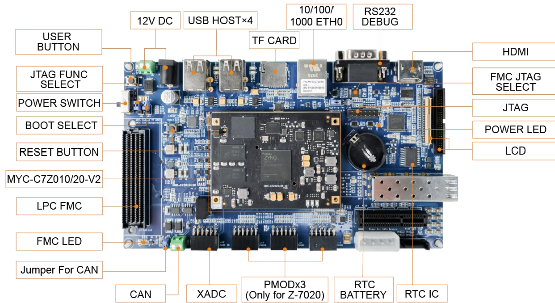
MYD-C7Z010/20-V2 Development Board
