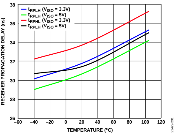
Figure 37. Receiver Propagation Delay vs. Temperature
