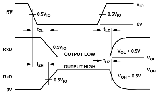
Figure 6. Receiver Enable or Disable Timing (See Figure 45 for Test Circuit)
