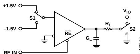
Figure 45. Receiver Enable or Disable Time Measurement
