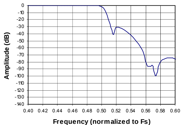
Figure 31. ADC Single-Speed Stopband Rejection
