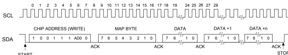
Figure 15. Control Port Timing, I²C Write
