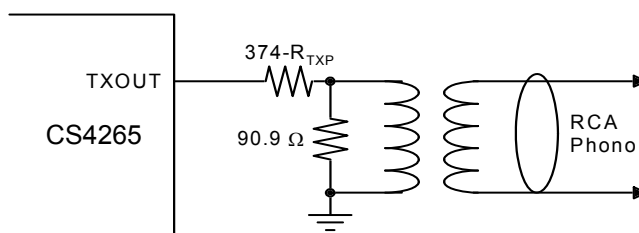
Figure 42. Consumer Output Circuit ( V_D = 5\text{ V} )
