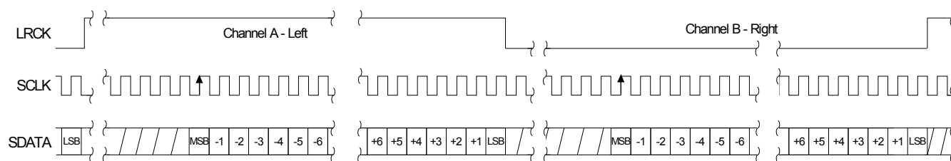
Figure 7. Format 2, Right-Justified 16-Bit Data. Format 3, Right-Justified 24-Bit Data.
