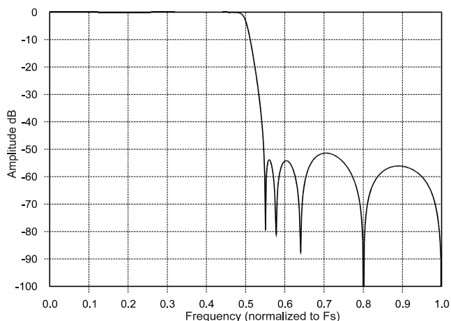
Figure 18. DAC Single-Speed Stopband Rejection
