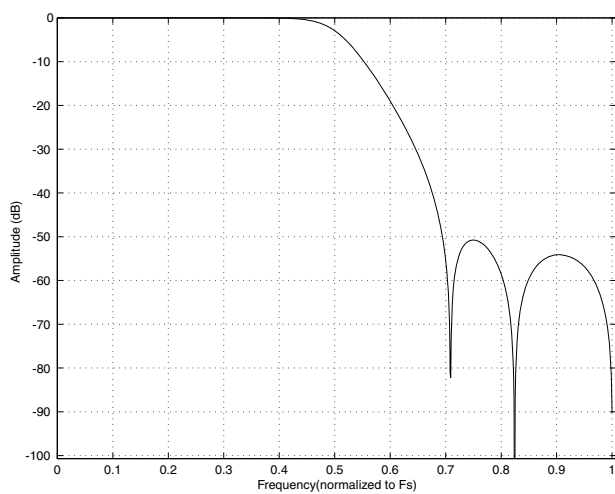
Figure 26. DAC Quad-Speed Stopband Rejection
