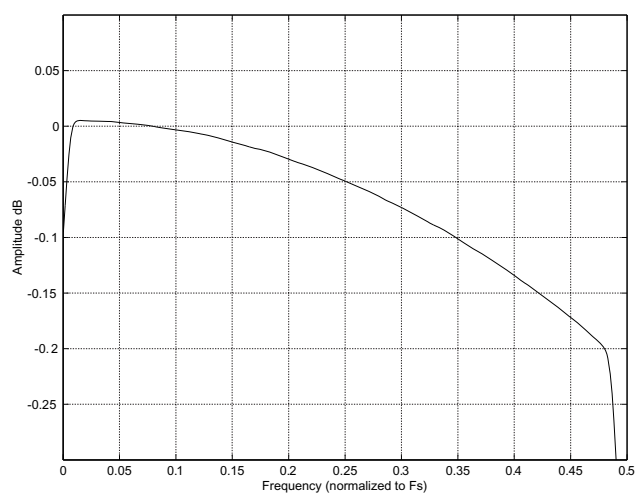
Figure 21. DAC Single-Speed Passband Ripple
