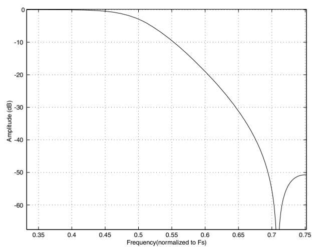
Figure 27. DAC Quad-Speed Transition Band
