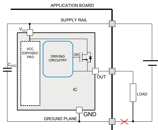
Figure 9. GND disconnection
