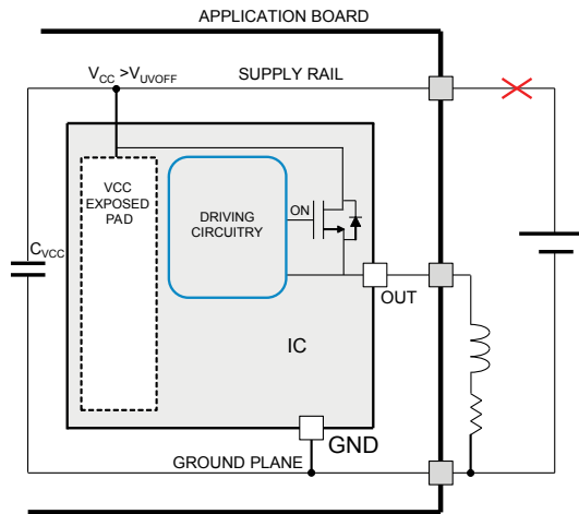
Figure 8. VCC disconnection
