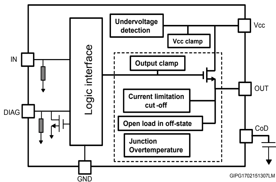
Figure 1. Block diagram
