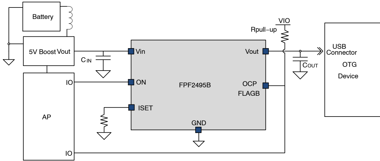
Figure 1. Typical Application
