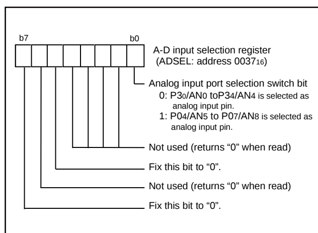
Fig. 43 Structure of A-D input selection register (spec. A)
