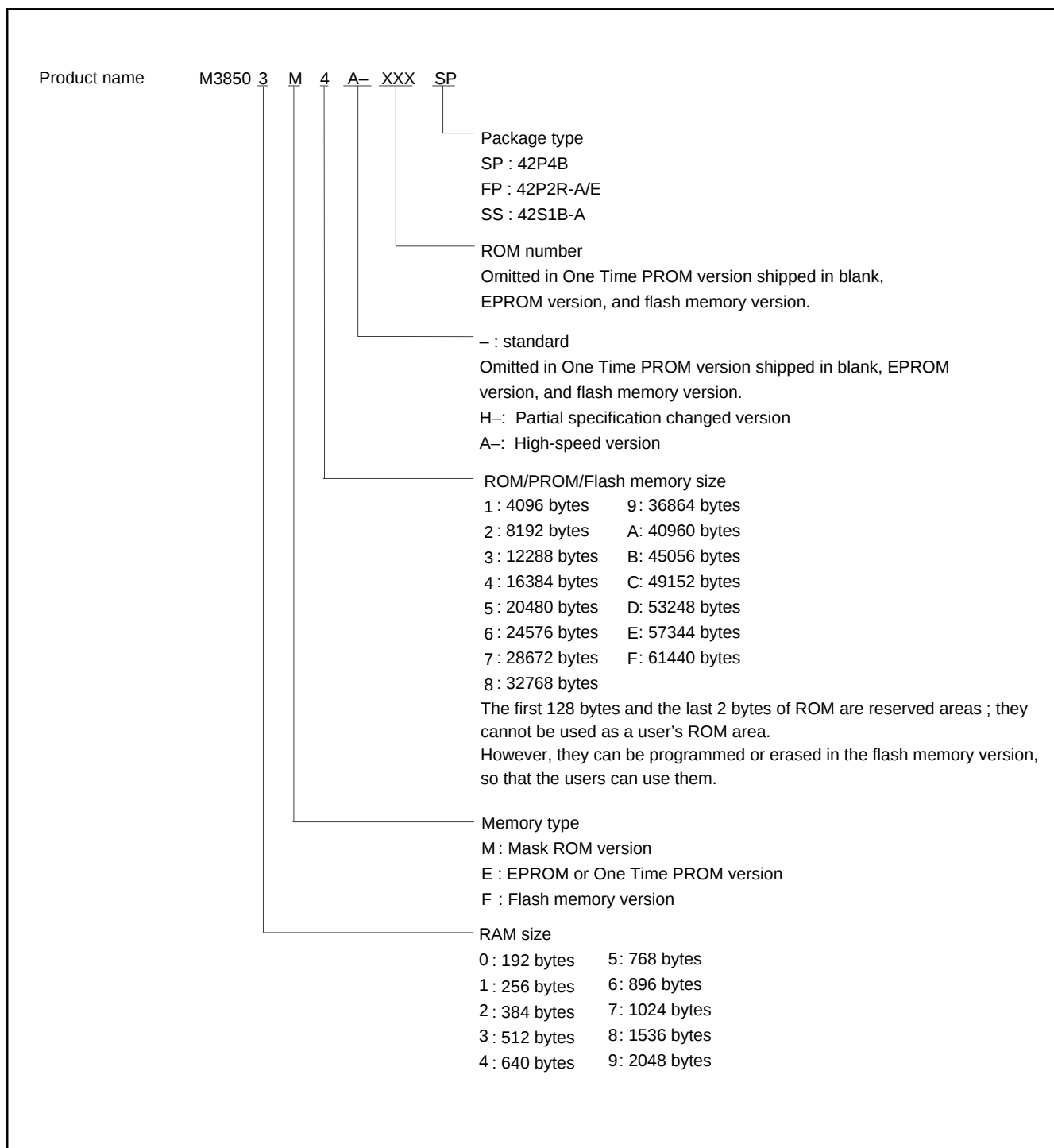
Fig. 5 Part numbering
