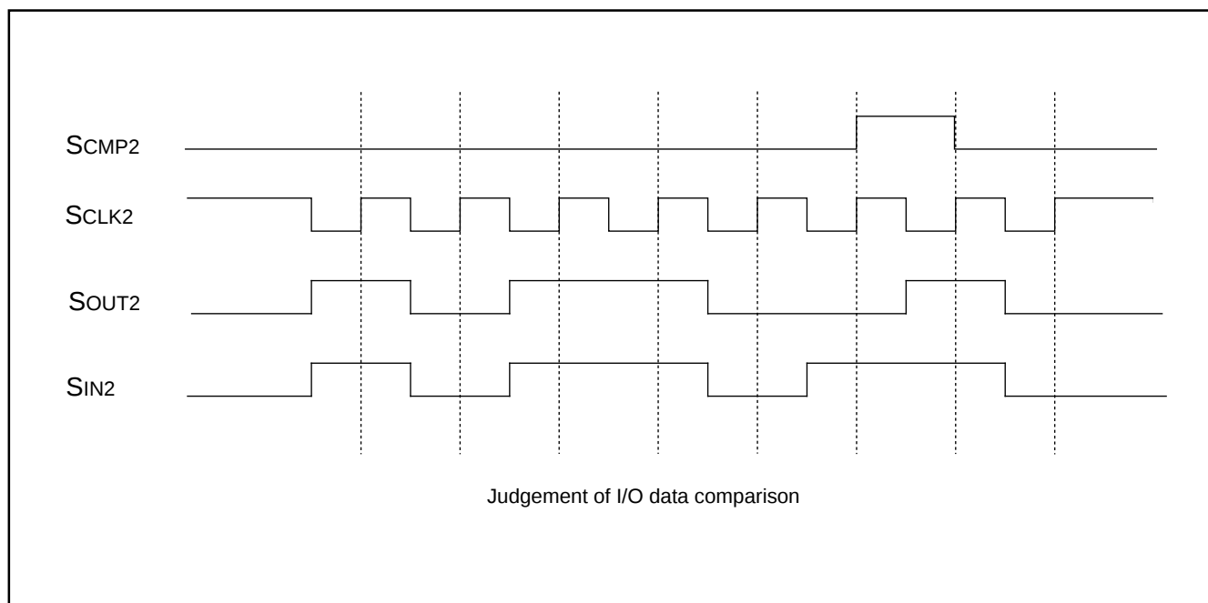
Fig. 34 SCMP2 output operation
