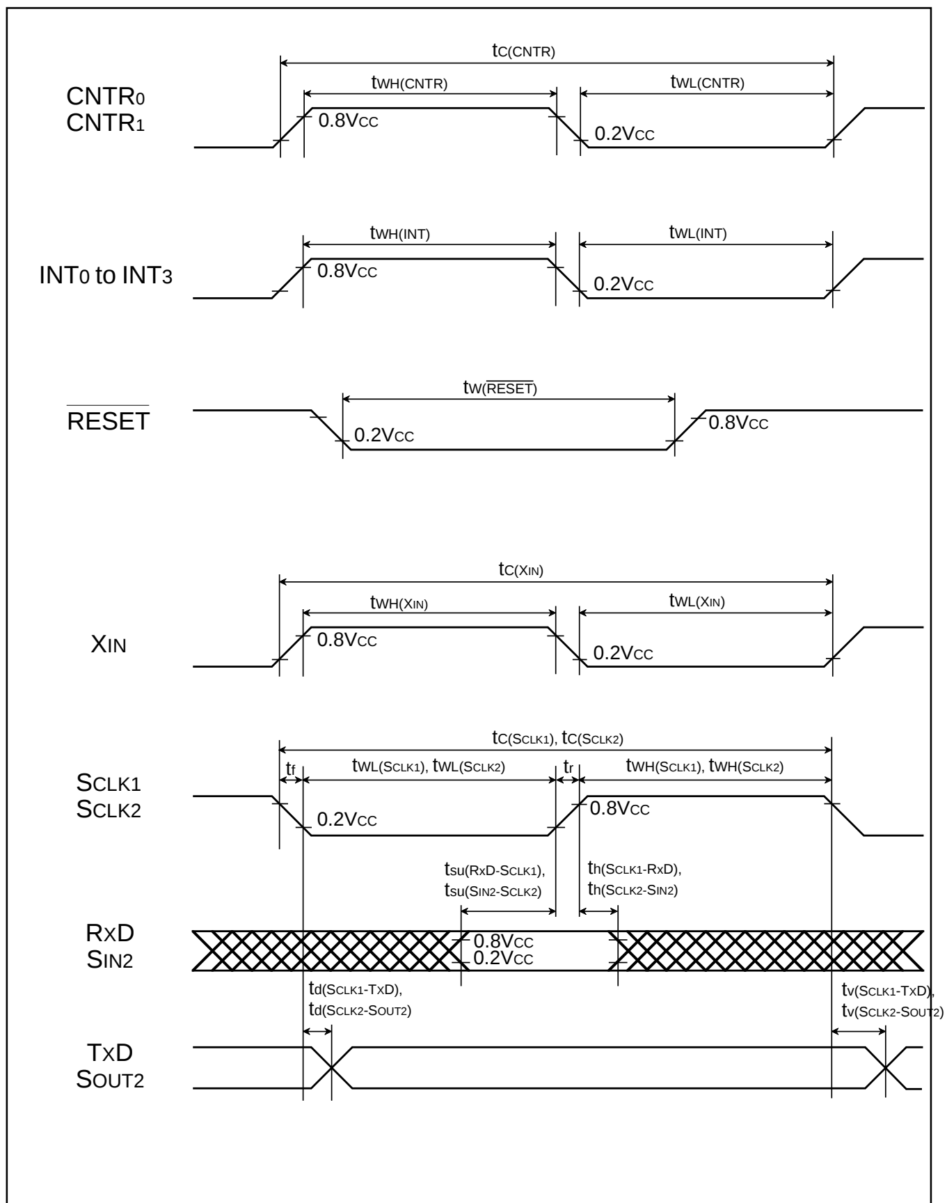
Fig. 79 Timing diagram
