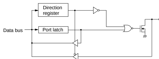
(8) Ports P22,P23
