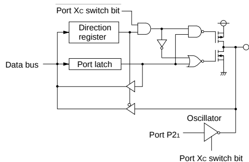
(8) Ports P22,P23
