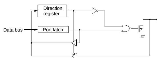
(8) Ports P22,P23
