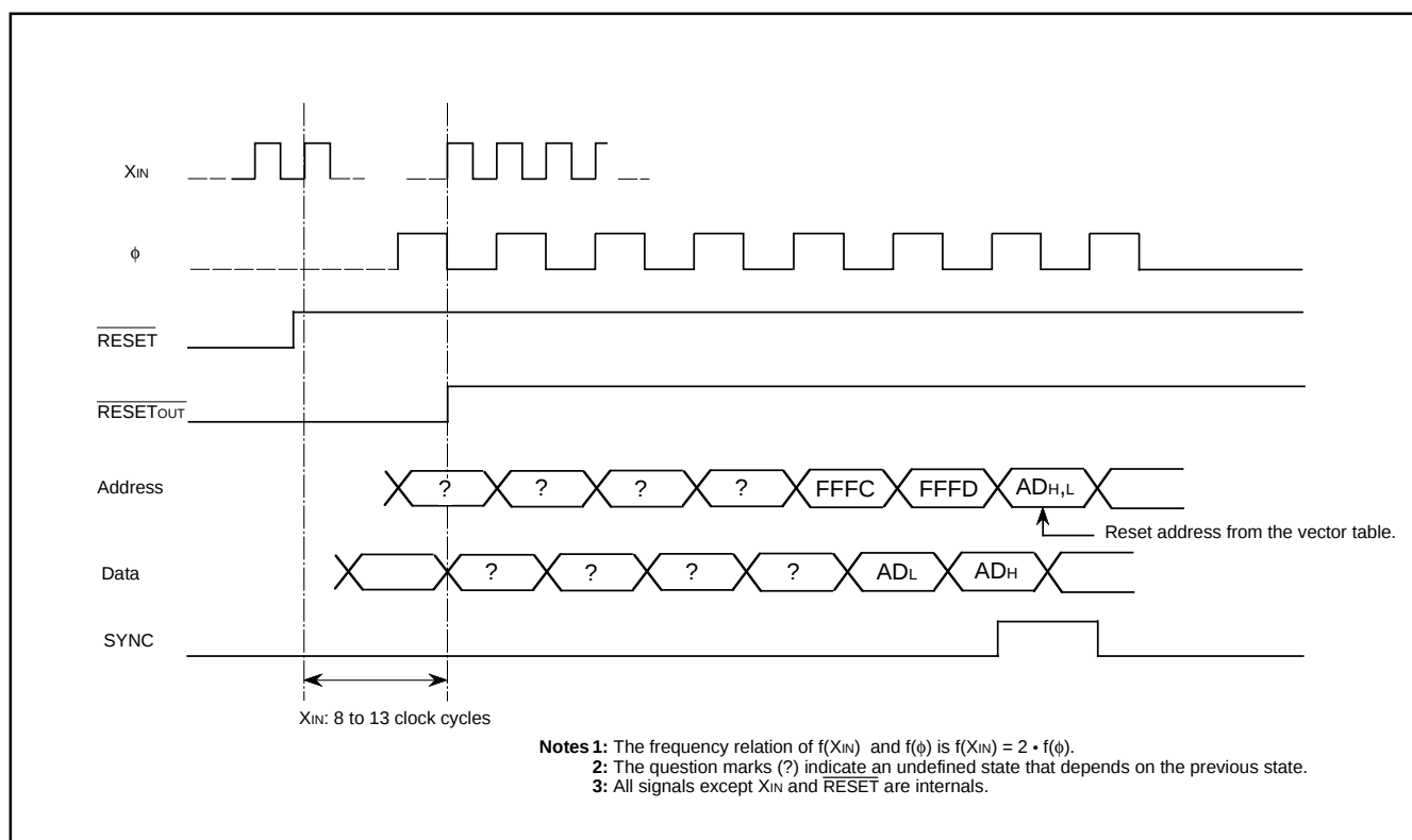
Fig. 49 Reset sequence
