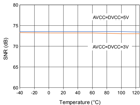
Figure 29. SNR vs. temperature
