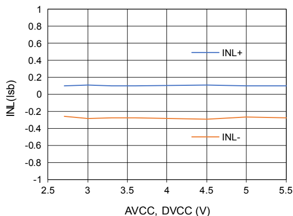
Figure 11. +/- INL vs. AVCC = DVCC
