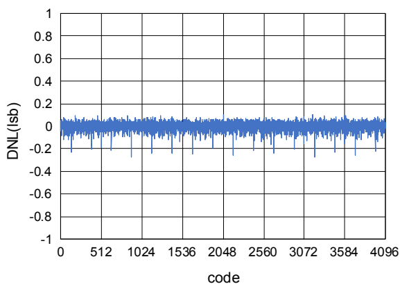
Figure 6. DNL vs. output codes (AVCC = DVCC = 3 V)
