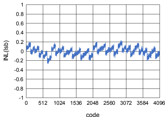
Figure 9. INL vs. output codes (AVCC = DVCC = 5 V)
