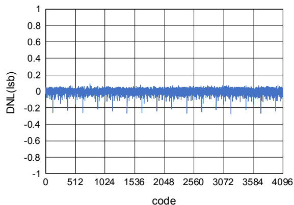
Figure 7. DNL vs. output codes (AVCC = DVCC = 5 V)
