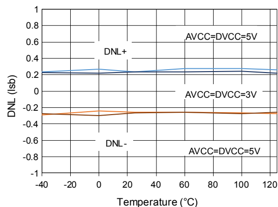
Figure 27. +/- DNL vs. temperature
