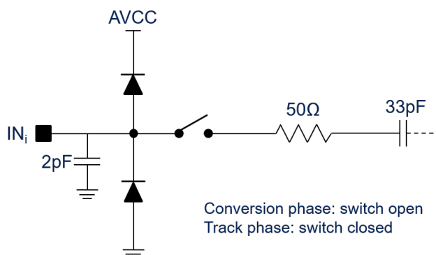
Figure 38. Equivalent input circuit
