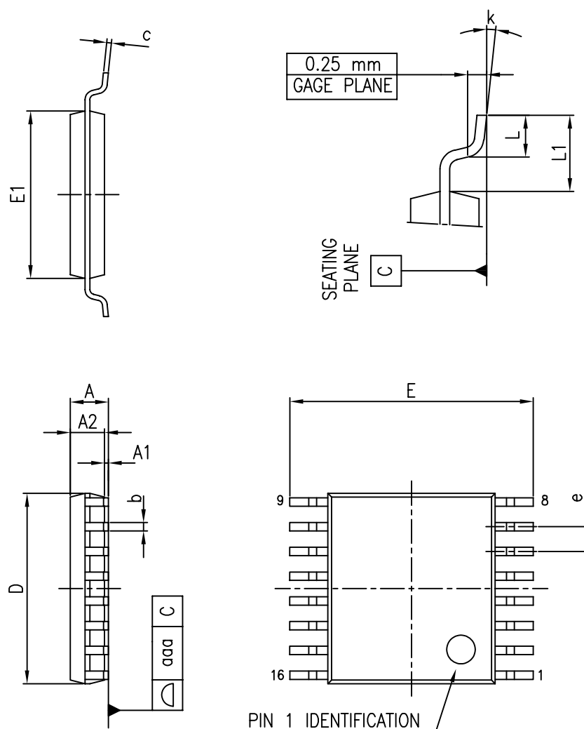
Figure 39. TSSOP-16 package outline
