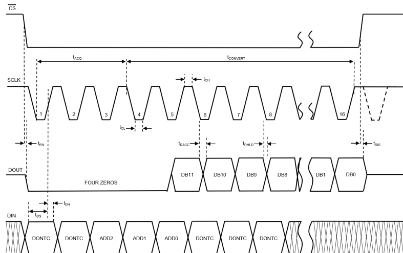
Figure 4. Serial timing diagram
