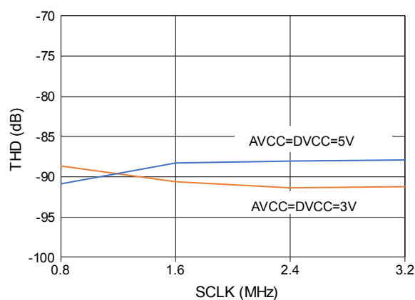
Figure 25. THD vs. SCLK
