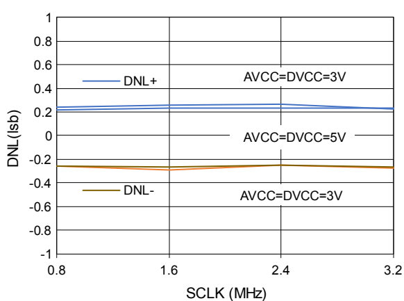
Figure 22. +/- DNL vs. SCLK
