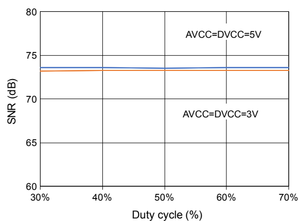
Figure 19. SNR vs. SCLK duty cycle
