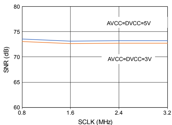
Figure 24. SNR vs. SCLK
