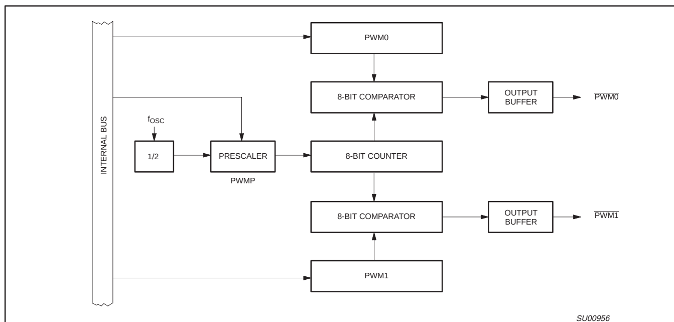
Figure 19. Functional Diagram of Pulse Width Modulated Outputs
