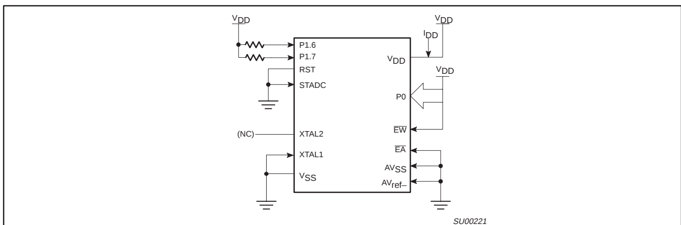
Figure 61. I_{DD} Test Condition, Power Down Mode All other pins are disconnected. V_{DD} = 2\text{ V to } 5.5\text{ V}^3
