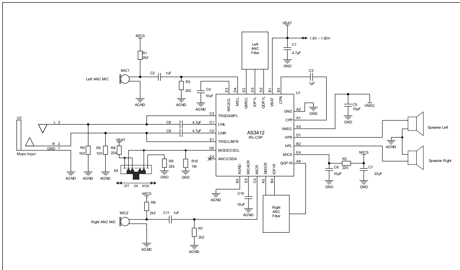
Figure 91: Full Slider Operation Mode – Application Example
