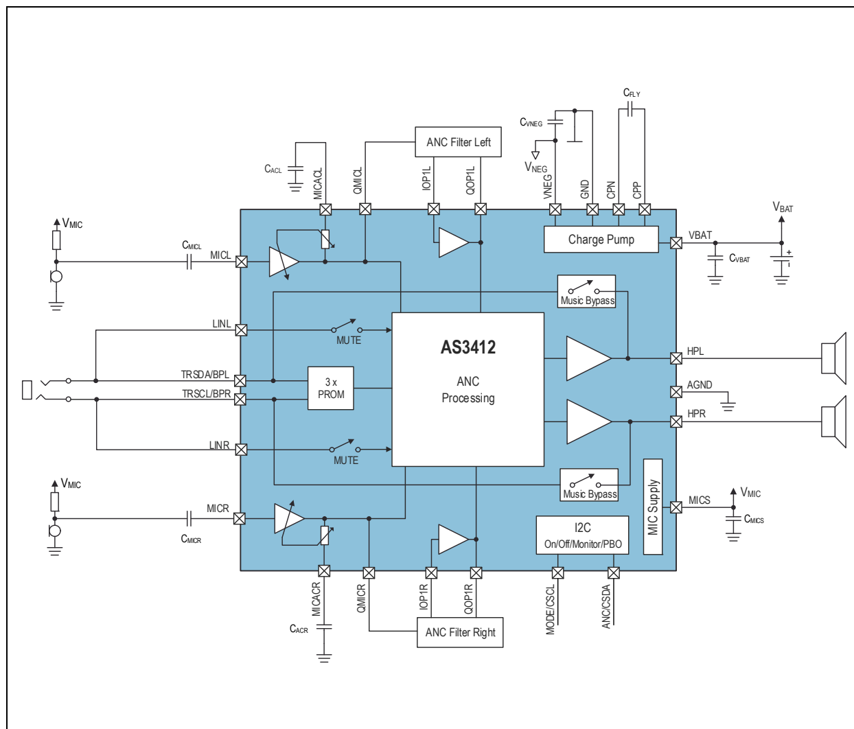
Figure 2: Functional Blocks of AS3412
