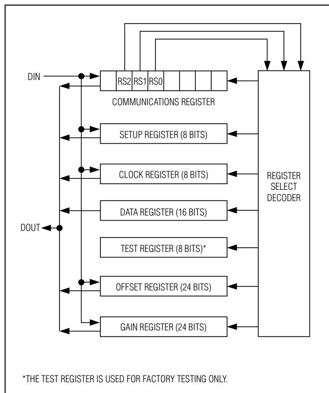
Figure 10. Register Summary
