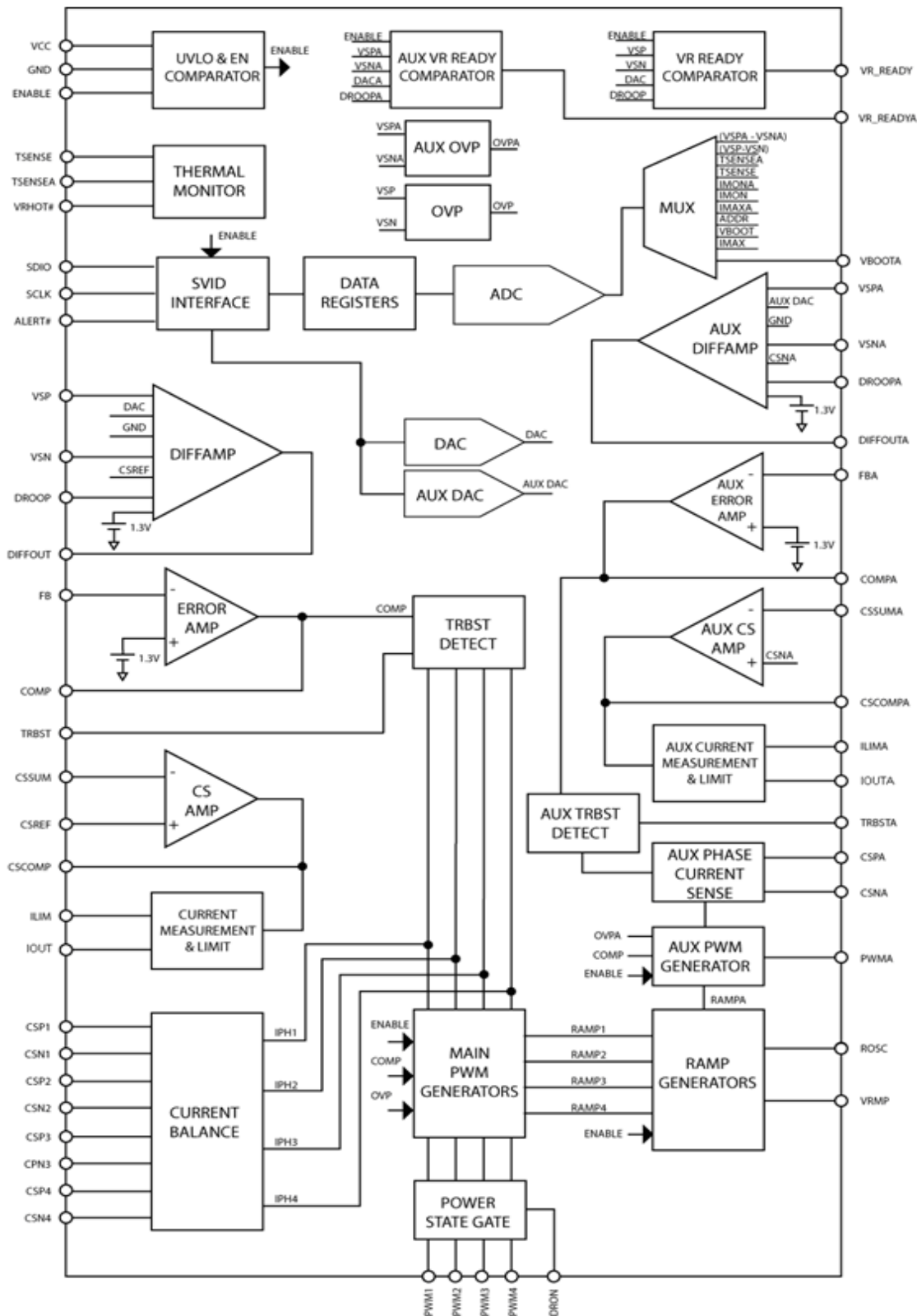
Figure 1. Block Diagram
