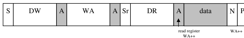
Figure 3 – I^2C Random-Read:
