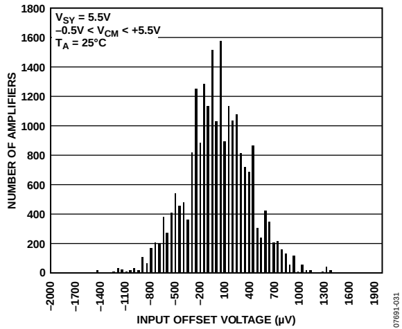
Figure 31. Amplifier Input Offset Voltage Distribution
