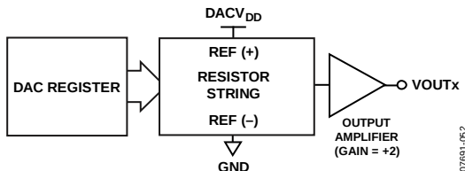
Figure 52. DAC Architecture
