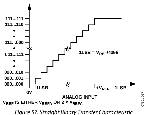
Figure 57. Straight Binary Transfer Characteristic
