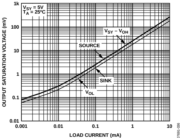
Figure 36. Amplifier Output Saturation Voltage vs. Load Current
