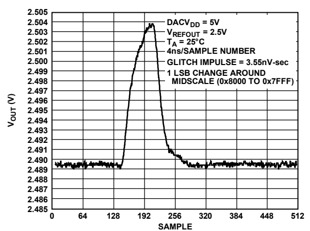
Figure 17. DAC Digital-to-Analog Glitch Impulse (Negative)
