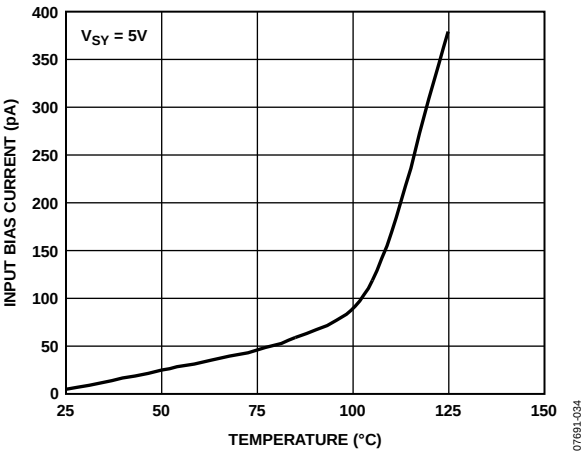
Figure 34. Amplifier Input Bias Current vs. Temperature
