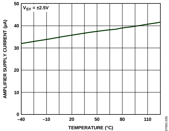
Figure 35. Amplifier Supply Current vs. Temperature
