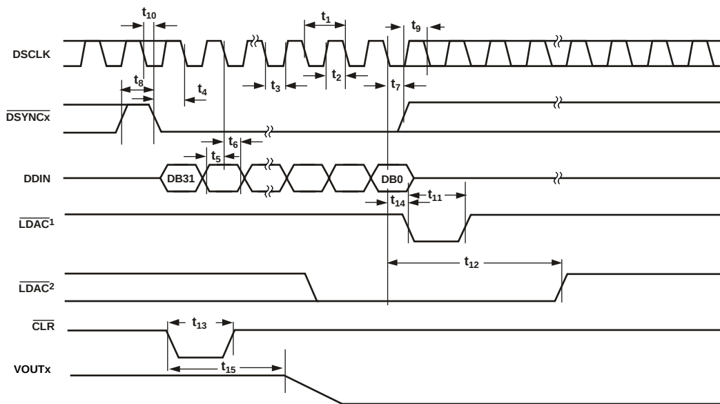
Figure 4. DAC Timing Characteristics
