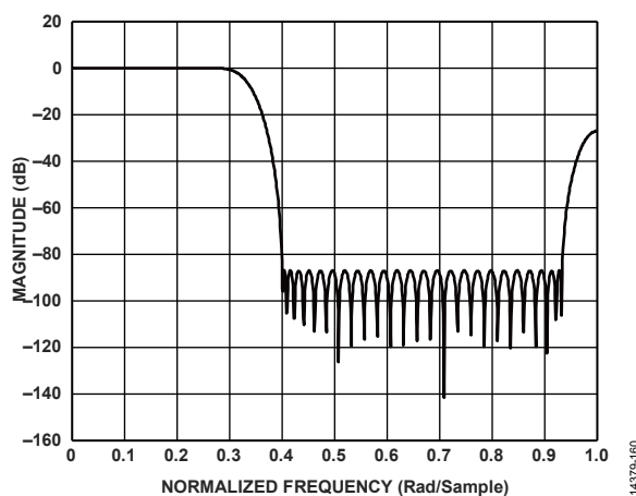
Figure 166. 3x Third-Band 80% Filter Response
