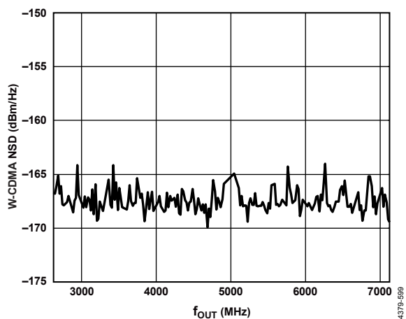
Figure 99. W-CDMA NSD vs. f_{OUT}
