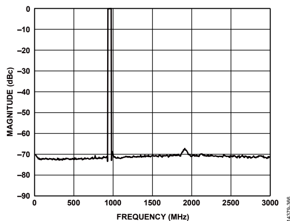
Figure 44. Eight Carriers at 950 MHz Output
