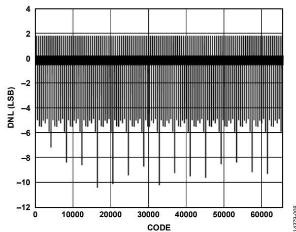
Figure 61. DNL, I_{OUTFS} = 20\text{ mA}
