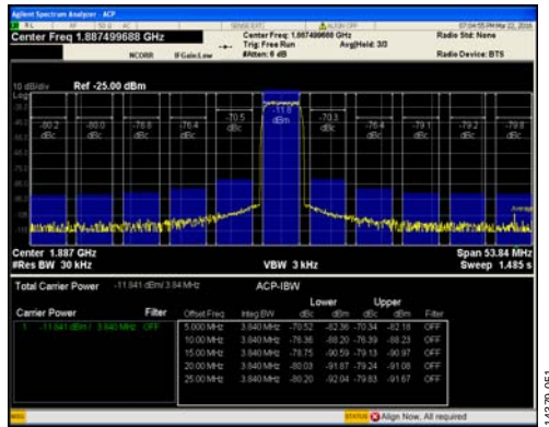
Figure 106. Single-Carrier W-CDMA at 1887.5 MHz
