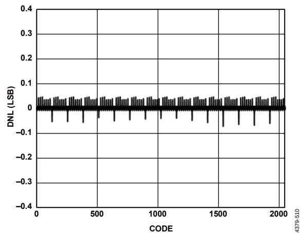
Figure 11. DNL, I_{OUTFS} = 40 mA
