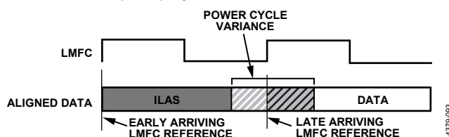
Figure 155. Link Delay &gt; LMFC Period Example
