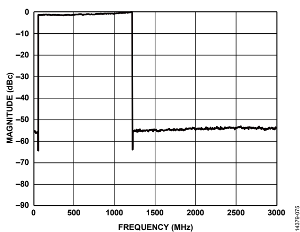
Figure 135. 194-Carrier, Sinc Enabled, FIR85 Enabled
