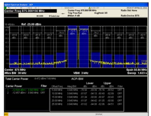
Figure 87. Two-Carrier W-CDMA at 875 MHz
