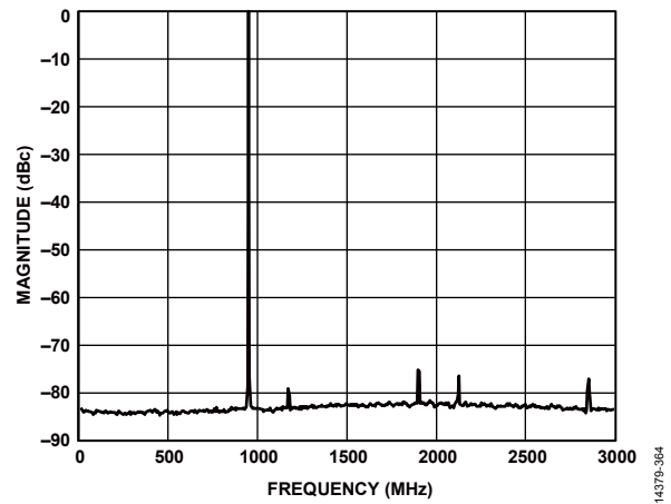
Figure 119. Single Carrier at 950 MHz Output (Shuffle On)
