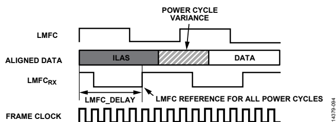
Figure 156. LMFC_DELAY_x to Compensate for Link Delay &gt; LMFC
