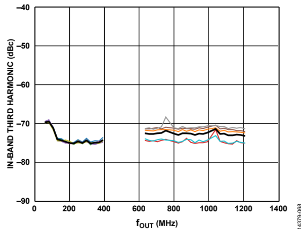
Figure 128. In-Band Third Harmonic vs. f_{OUT} Performance for Four DOCSIS Carriers
