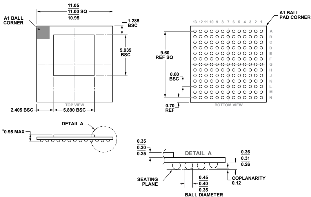
Figure 195. 165-Ball Chip Scale Package Ball Grid Array [CSP_BGA] (BC-165-1)
