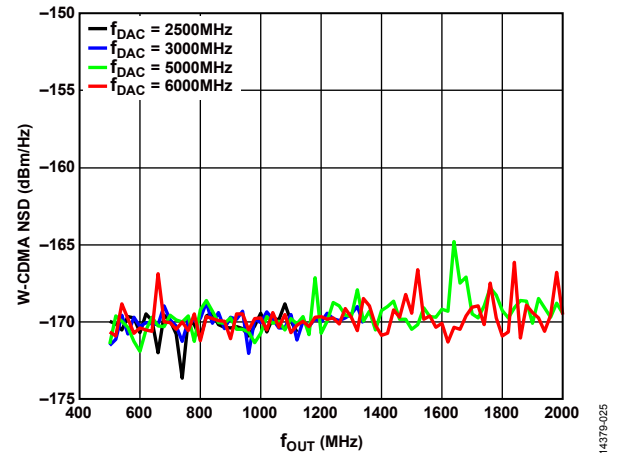
Figure 79. W-CDMA NSD Measured at 70 MHz vs. f_{OUT} over f_{DAC}
