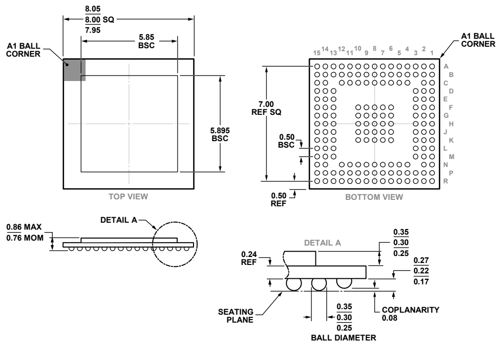
Figure 195. 165-Ball Chip Scale Package Ball Grid Array [CSP_BGA] (BC-165-1)
