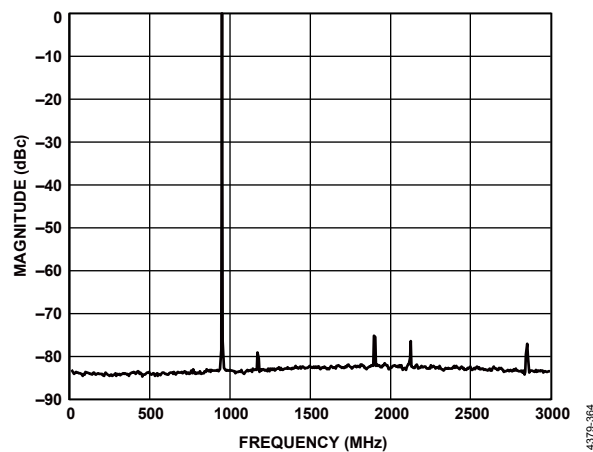
Figure 42. Single Carrier at 950 MHz Output
