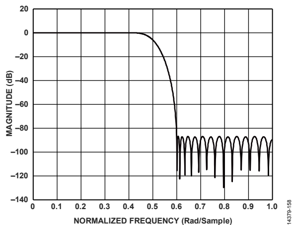
Figure 164. First 2x Half-Band 80% Filter Response
