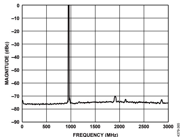
Figure 43. Four Carriers at 950 MHz Output
