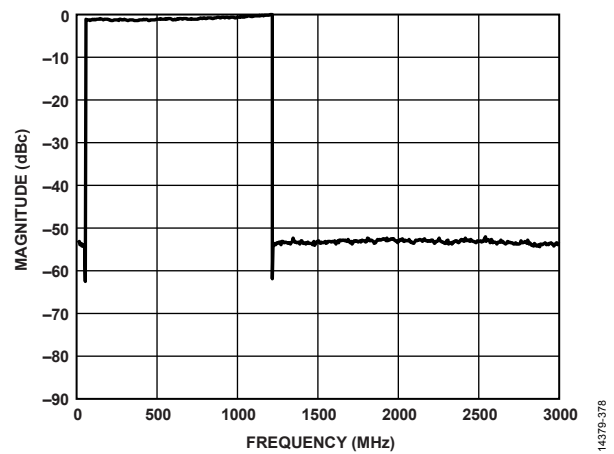
Figure 56. 194-Carrier, Sinc On, FIR85 Enabled
