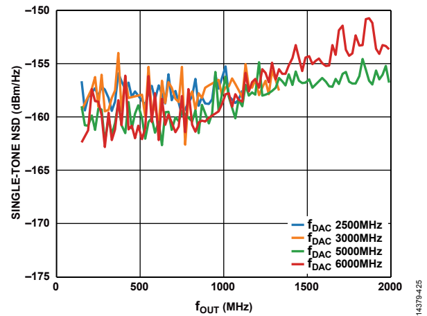
Figure 23. Single-Tone NSD Measured at 10% Offset from f_{OUT} vs. f_{OUT} over f_{DAC}
