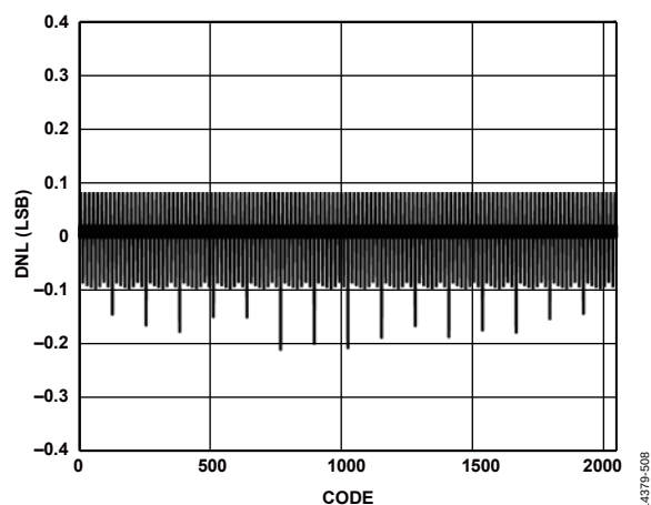
Figure 9. DNL, I_{OUTFS} = 20 mA
