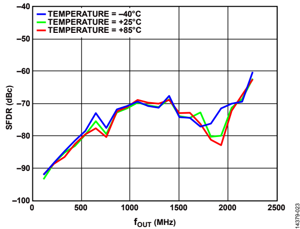
Figure 76. SFDR vs. f_{OUT} over Temperature
