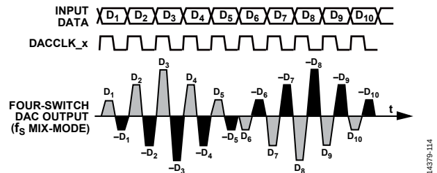
Figure 182. Mix-Mode Waveform
