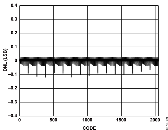
Figure 10. DNL, I_{OUTFS} = 30 mA
