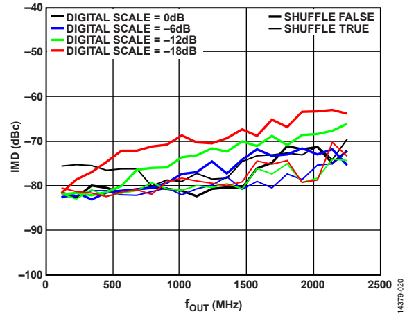
Figure 73. IMD vs. f_{OUT} over Digital Scale
