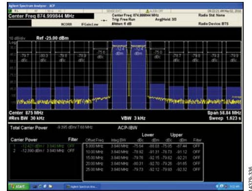
Figure 27. Two-Carrier W-CDMA at 875 MHz
