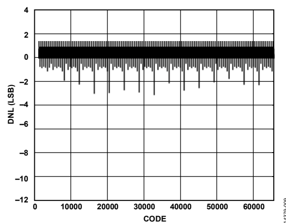
Figure 62. DNL, I_{OUTFS} = 30\text{ mA}
