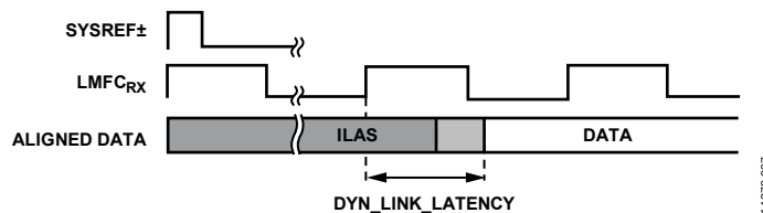
Figure 158. DYN_LINK_LATENCY_x Illustration
