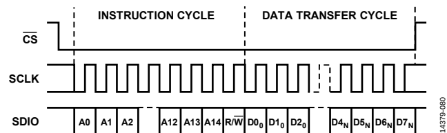
Figure 140. Serial Register Interface Timing, LSB First, Register 0x000, Bit 5 and Bit 2 = 1
