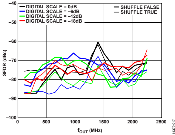
Figure 70. SFDR vs. f_{OUT} over Digital Scale
