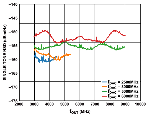
Figure 30. Single-Tone NSD Measured at 70\text{ MHz} vs. f_{OUT}
