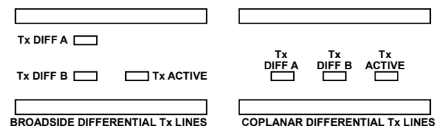
Figure 177. Broadside vs. Coplanar Differential Stripline Routing Techniques
