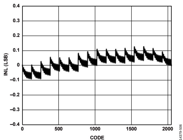
Figure 7. INL, I_{OUTFS} = 30 mA
