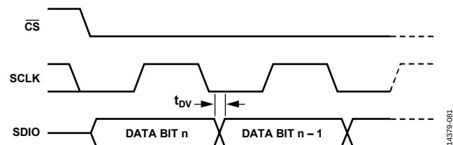
Figure 141. Timing Diagram for Serial Port Register Read
