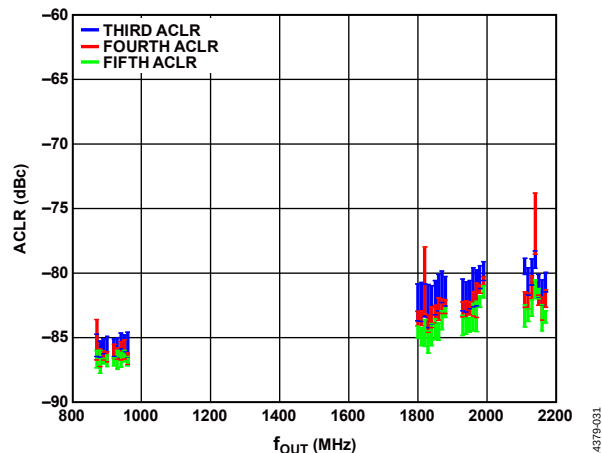
Figure 89. Single-Carrier, W-CDMA ACLR vs. f_{OUT} (Third ACLR, Fourth ACLR, Fifth ACLR)
