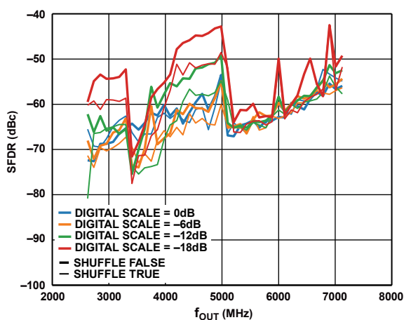
Figure 33. SFDR vs. f_{OUT} over Digital Full Scale
