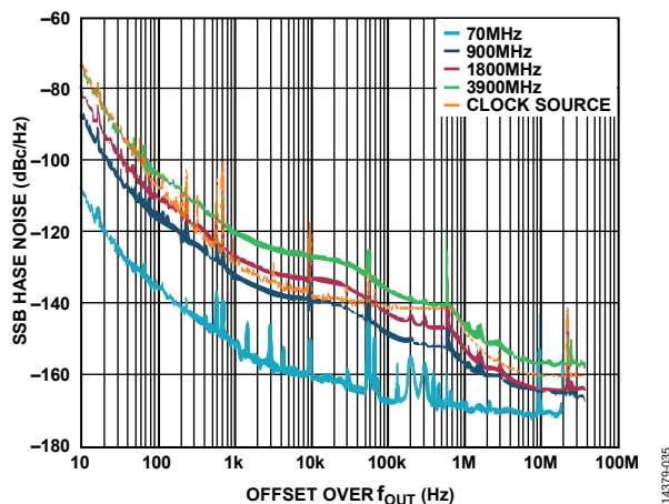
Figure 90. SSB Phase Noise vs. Offset over f_{OUT} , f_{DAC} = 4000 \text{ MSPS} (Two Different DAC Clock Sources Used for Best Composite Curve)
