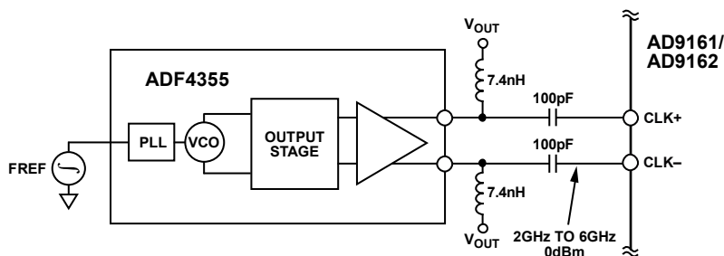
Figure 186. Possible Signal Chain for \text{CLK}^{\pm} Input
