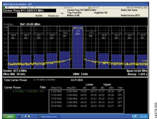
Figure 25. Single-Carrier W-CDMA at 877.5 MHz
