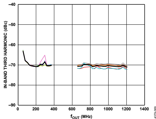
Figure 129. In-Band Third Harmonic vs. f_{OUT} Performance for Eight DOCSIS Carriers
