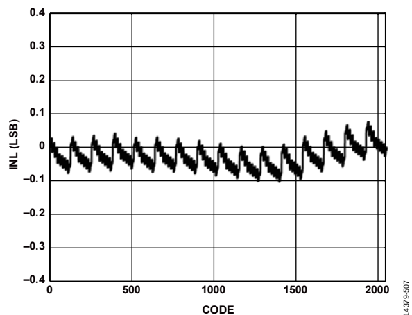
Figure 8. INL, I_{OUTFS} = 40 mA
