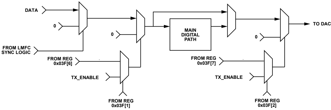
Figure 174. Downstream Protection Block Diagram
