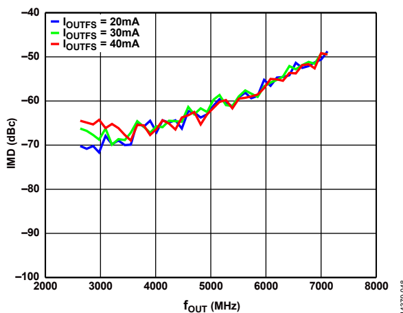
Figure 104. IMD vs. f_{OUT} over DAC I_{OUTFS}
