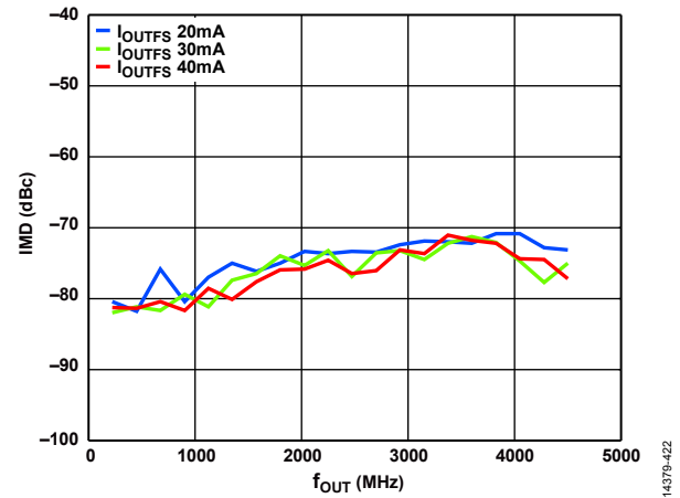
Figure 22. IMD vs. f_{OUT} over DAC I_{OUTFS}
