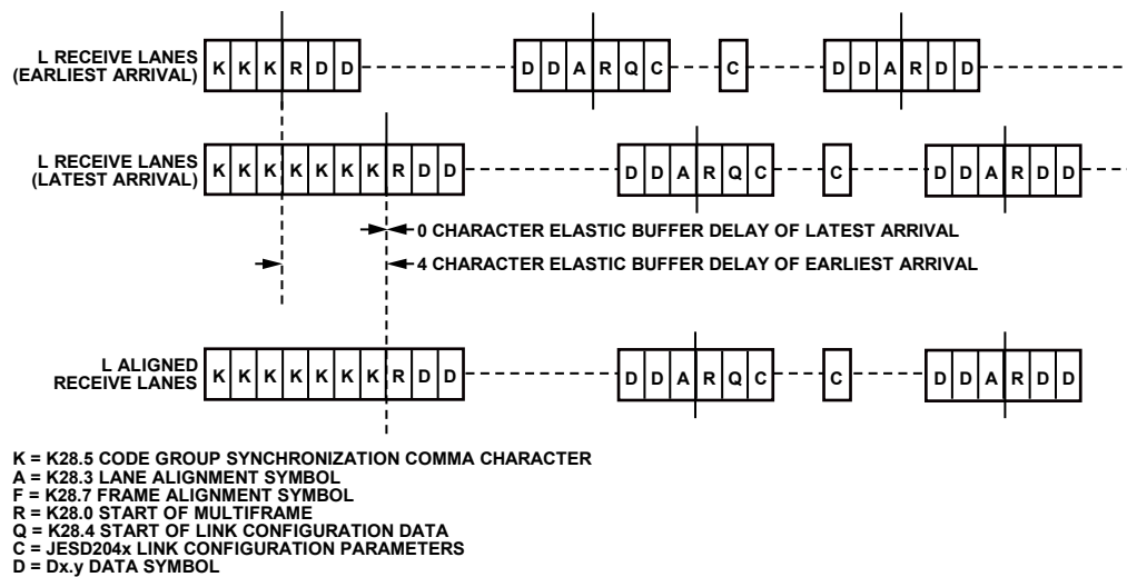
Figure 151. Lane Alignment During ILAS
