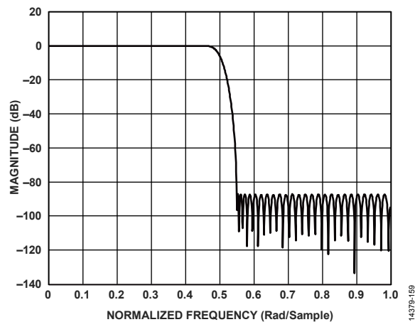
Figure 165. First 2x Half-Band 90% Filter Response
