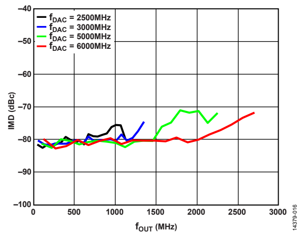
Figure 69. IMD vs. f_{OUT} over f_{DAC}
