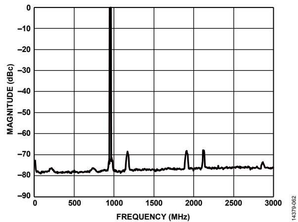
Figure 120. Four Carriers at 950 MHz Output
