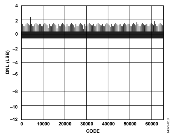
Figure 63. DNL, I_{OUTFS} = 40\text{ mA}
