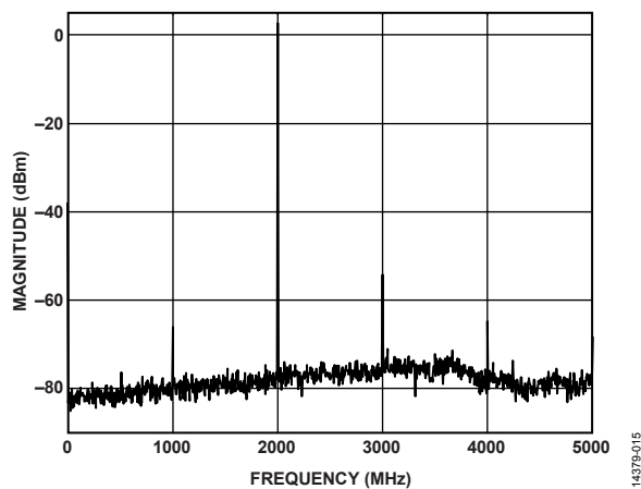
Figure 68. Single-Tone Spectrum at f_{OUT} = 2000\text{ MHz} (FIR85 Enabled)
