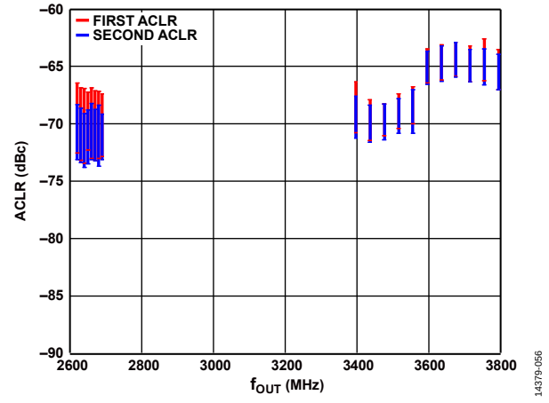
Figure 110. Four-Carrier, W-CDMA ACLR vs. f_{OUT} (First ACLR, Second ACLR)
