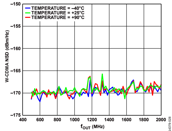
Figure 85. W-CDMA NSD Measured at 70 MHz vs. f_{OUT} over Temperature
