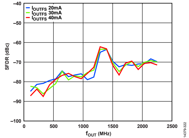
Figure 21. SFDR vs. f_{OUT} over DAC I_{OUTFS}
