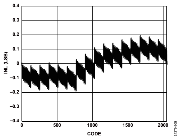
Figure 6. INL, I_{OUTFS} = 20 mA
