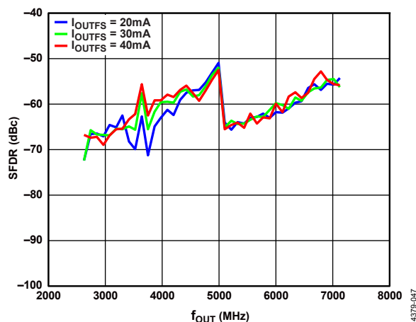
Figure 103. SFDR vs. f_{OUT} over DAC I_{OUTFS}
