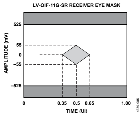
Figure 145. Receiver Eye Mask for 600 mV V_{TT} Swing
