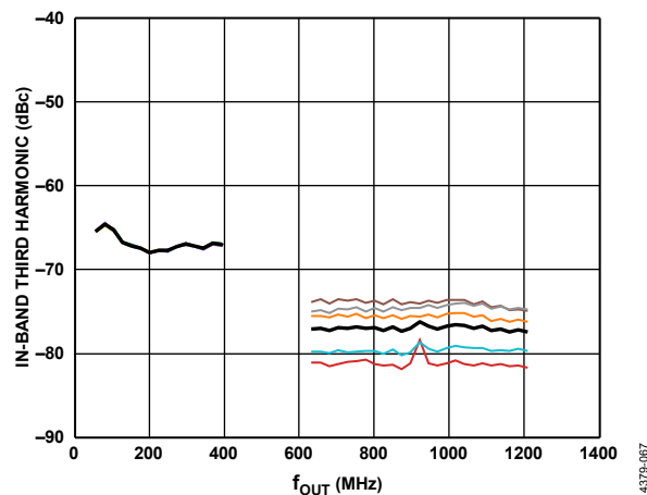
Figure 127. In-Band Third Harmonic vs. f_{OUT} Performance for One DOCSIS Carrier
