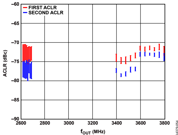
Figure 107. Single-Carrier, W-CDMA ACLR vs. f_{OUT} (First ACLR, Second ACLR)
