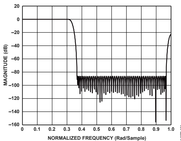
Figure 167. 3x Third-Band 90% Filter Response
