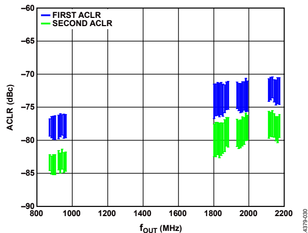
Figure 88. Single-Carrier, W-CDMA ACLR vs. f_{OUT} (First ACLR, Second ACLR)
