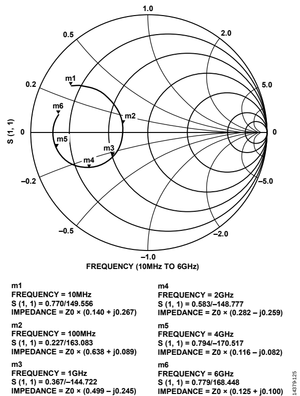
Figure 194. Simulated Smith Chart Showing the DAC Output Impedance ( Z_0 = 100 \Omega )
