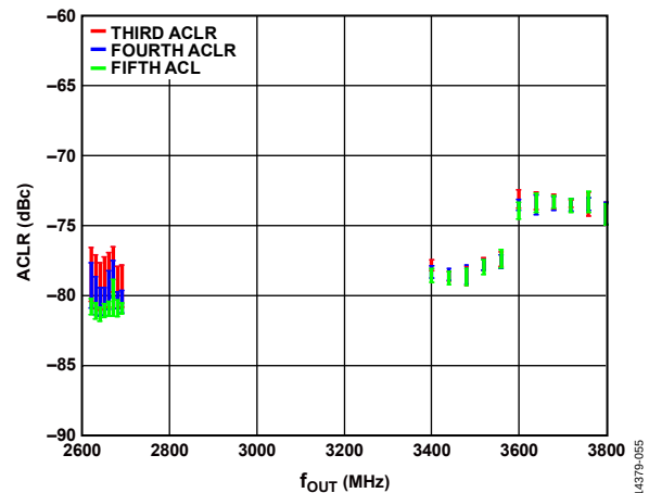
Figure 108. Single-Carrier, W-CDMA ACLR vs. f_{OUT} (Third ACLR, Fourth ACLR, Fifth ACLR)
