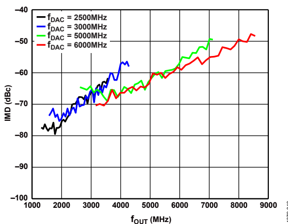
Figure 105. IMD vs. f_{OUT} over f_{DAC}
