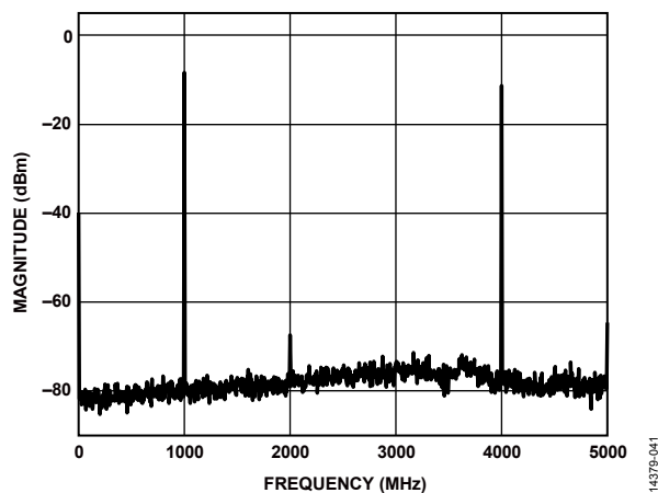
Figure 97. Single-Tone Spectrum at f_{OUT} = 4000\text{ MHz}
