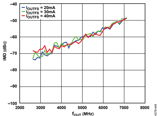
Figure 37. IMD vs. f_{OUT} over DAC I_{OUTFS}
