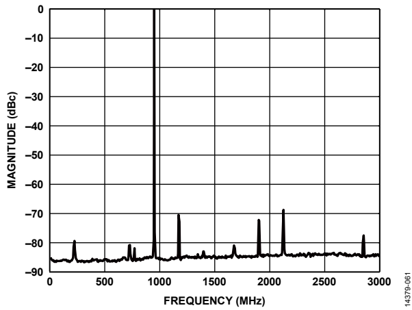
Figure 118. Single Carrier at 950 MHz Output
