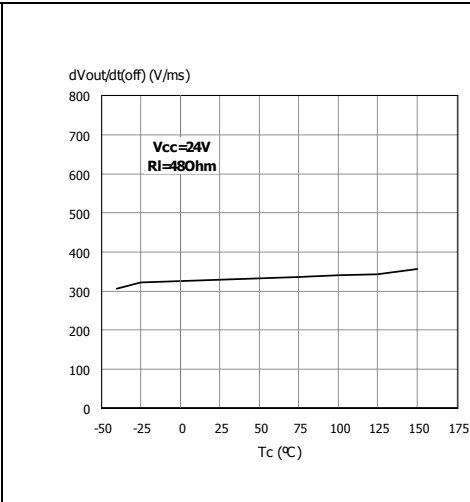
Figure 14. Turn-off voltage slope
