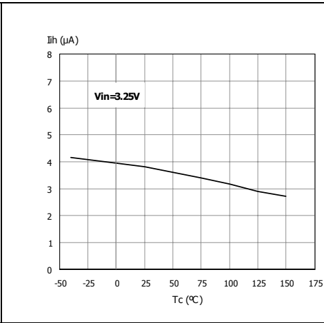
Figure 12. Status leakage current
