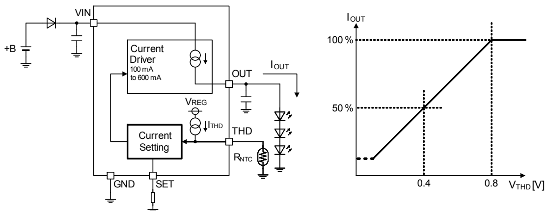
Thermal De-rating Function
