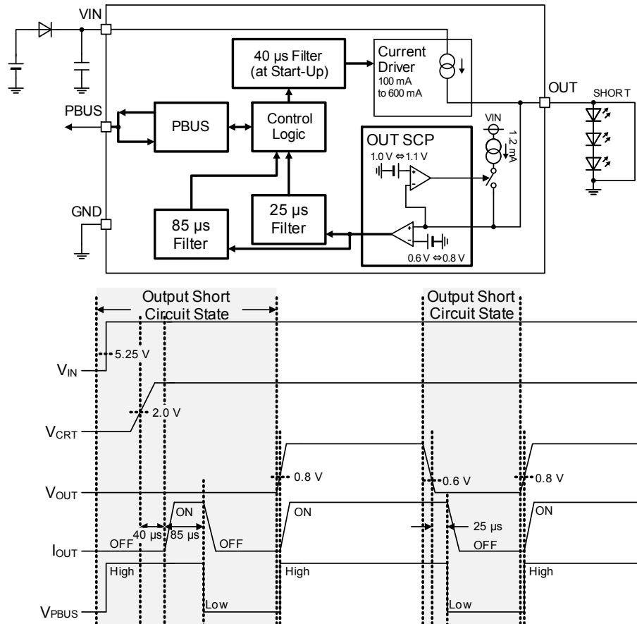
Output Short Circuit Protection (OUT SCP)
