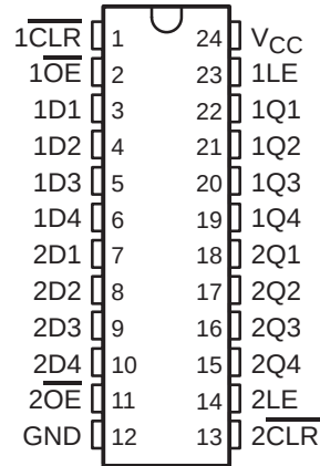
SN54ALS873B, SN54AS873 . . . JT PACKAGE SN74ALS873B, SN74AS873A . . . DW OR NT PACKAGE (TOP VIEW)
