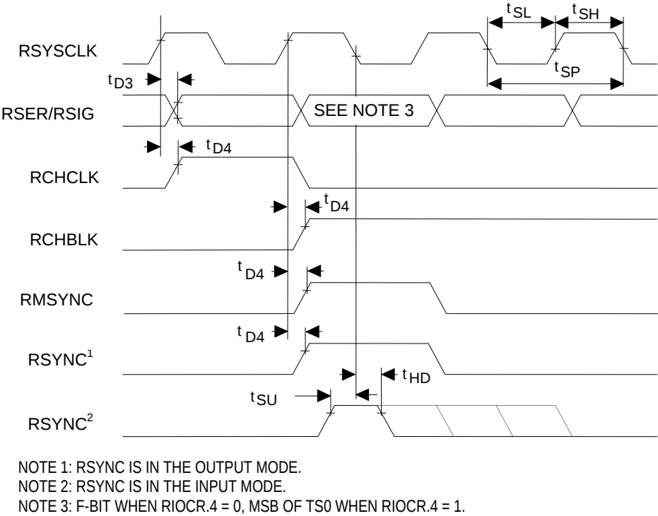
Figure 12-8. Receive Framing Timing—Line Side
