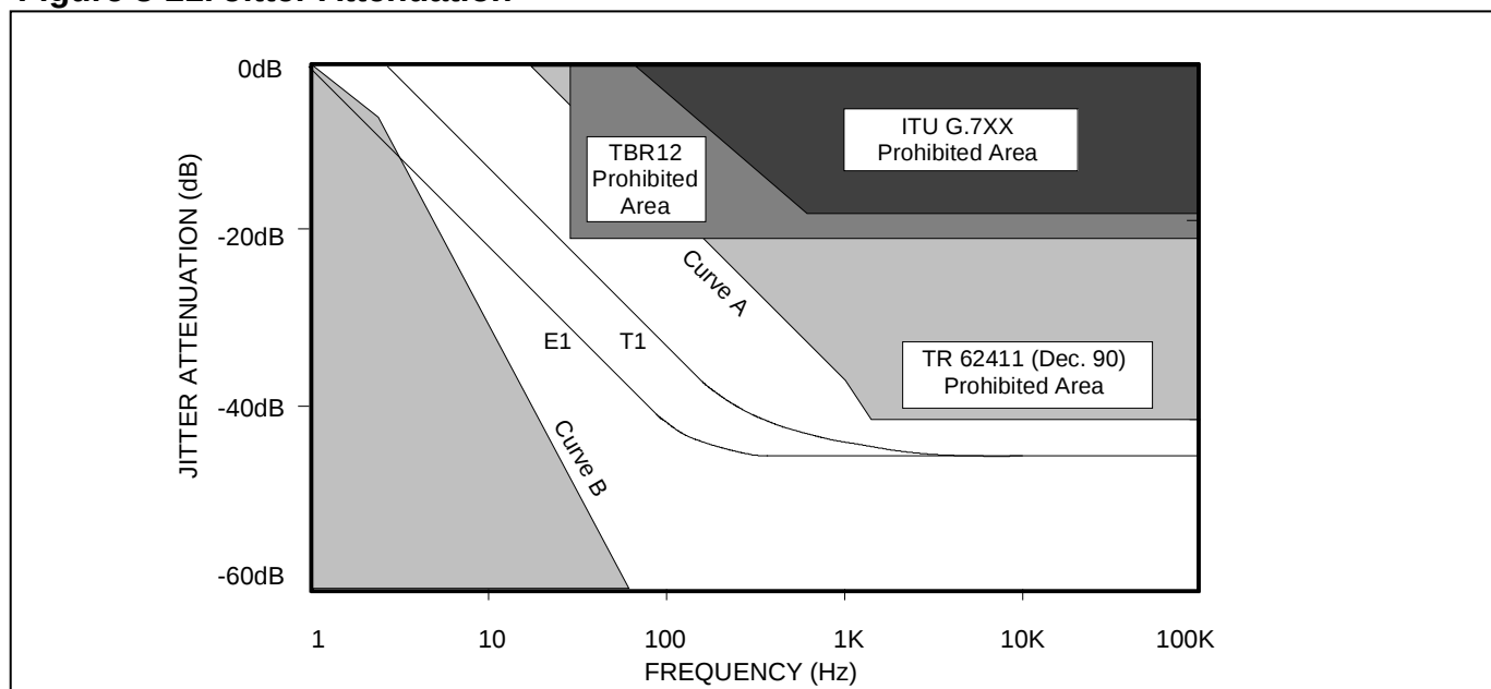
Figure 8-21. Jitter Attenuation
