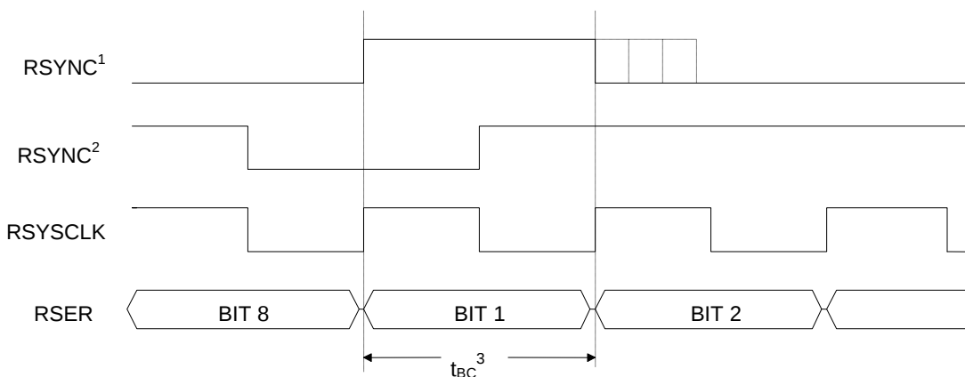
Figure 8-12. RSYNC Input in H.100 (CT Bus) Mode
