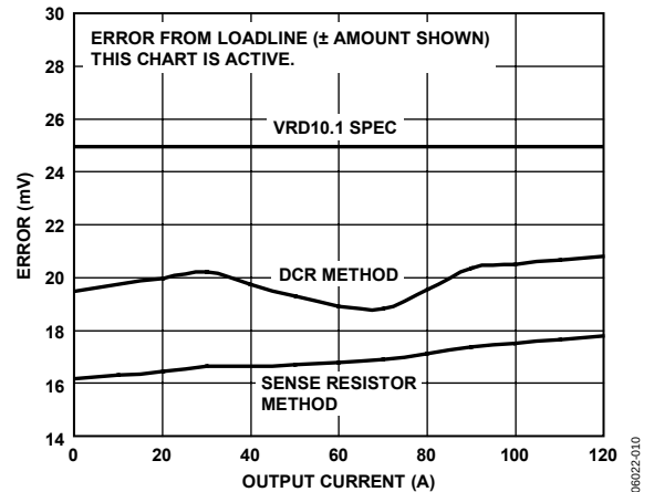
Figure 10. Accuracy Comparison of DCR and Sense Resistor Methods
