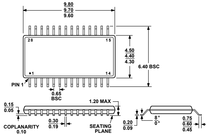
COMPLIANT TO JEDEC STANDARDS MO-153-AE Figure 21. 28-Lead Thin Shrink Small Outline Package [TSSOP] (RU-28) Dimensions shown in millimeters
