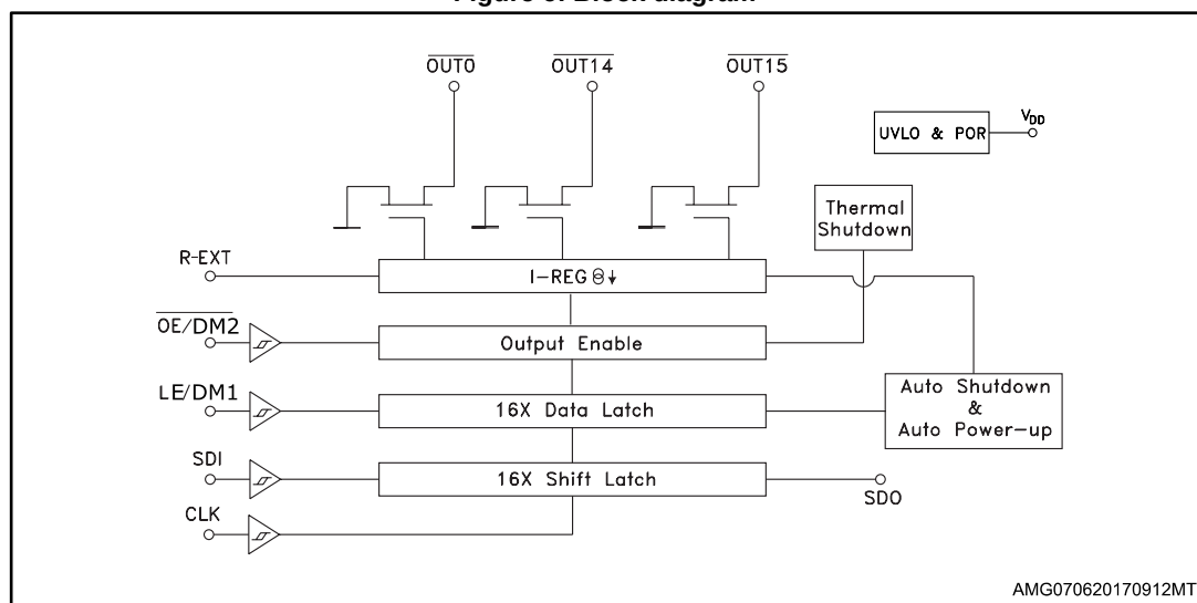
Figure 6: Block diagram
