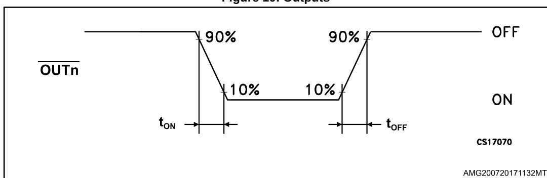
Figure 10: Outputs
