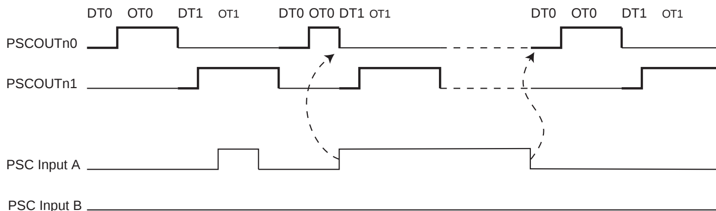
Figure 15-22. PSCn behaviour versus PSCn Input A in Fault Mode 2
