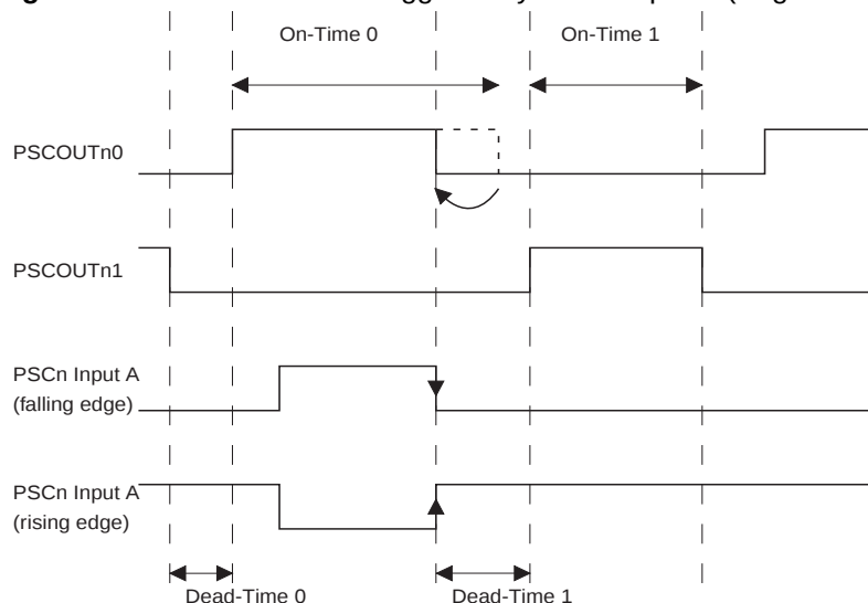
Figure 15-15. PSCOUTn0 retrigged by PSCn Input A (Edge Retriggering)
