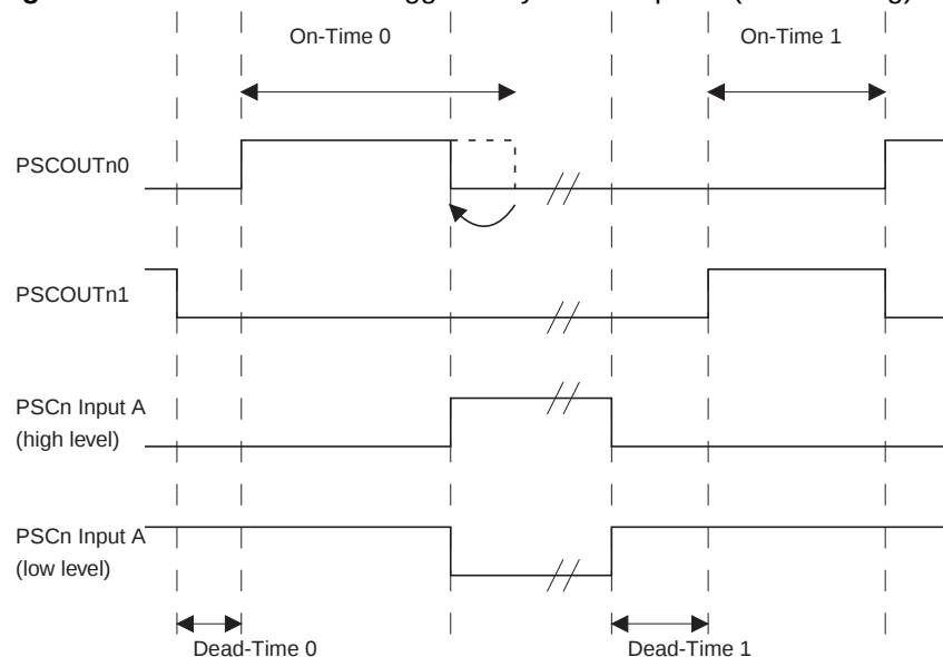
Figure 15-16. PSCOUTn0 retrigged by PSCn Input A (Level Acting)
