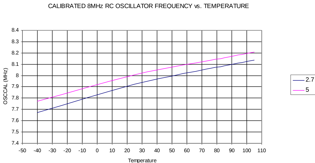
Figure 26-37. Calibrated 8 MHz RC Oscillator Frequency vs. Temperature
