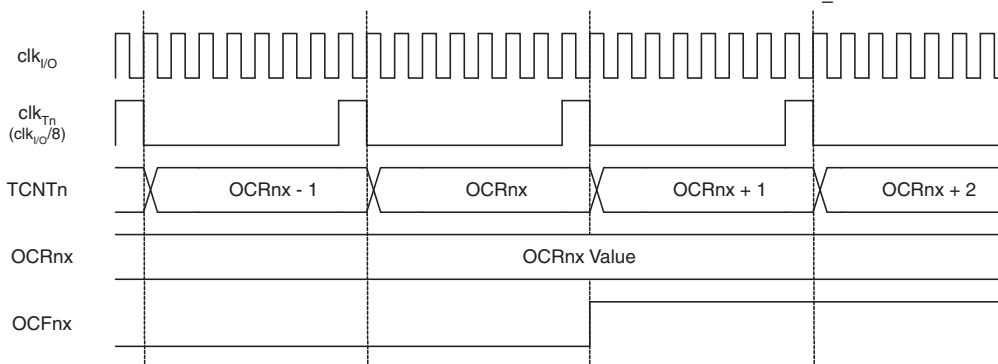
Figure 13-10. Timer/Counter Timing Diagram, Setting of OCF0x, with Prescaler ( f_{\text{clk\_I/O}}/8 )
