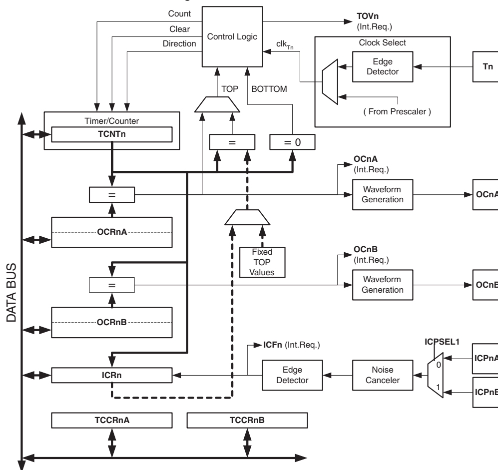
Figure 14-1. 16-bit Timer/Counter Block Diagram (1)
