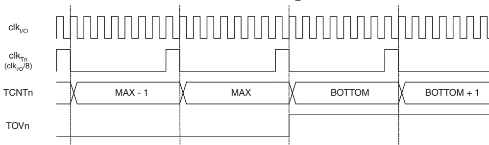
Figure 13-9. Timer/Counter Timing Diagram, with Prescaler ( f_{\text{clk\_I/O}}/8 )
