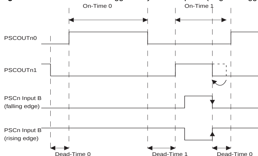
Figure 15-17. PSCOUTn1 retriggered by PSCn Input B (Edge Retriggering)
