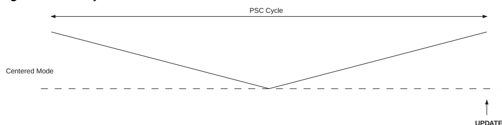
Figure 15-5. Cycle Presentation in Centered Mode
