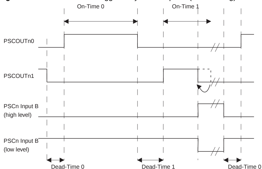
Figure 15-18. PSCOUTn1 retriggered by PSCn Input B (Level Acting)
