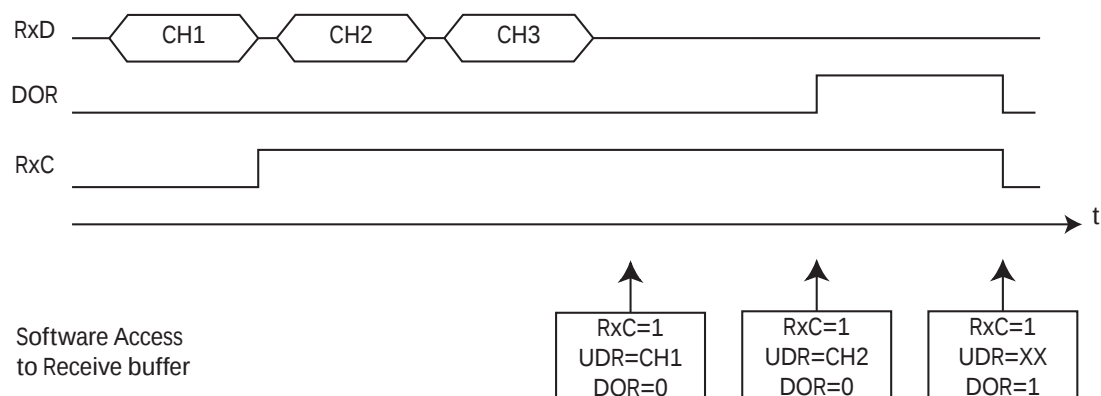
Figure 17-5. Data OverRun example
