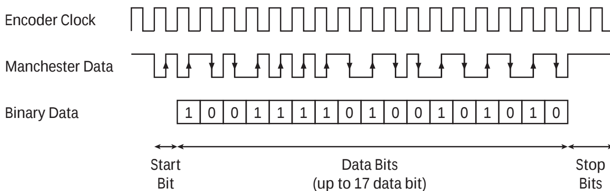
Figure 18-3. Manchester Frame example
