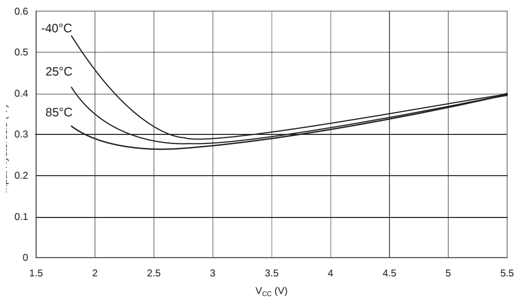
Figure 26-22. I/O Pin Input Hysteresis Voltage vs. V_{CC}
