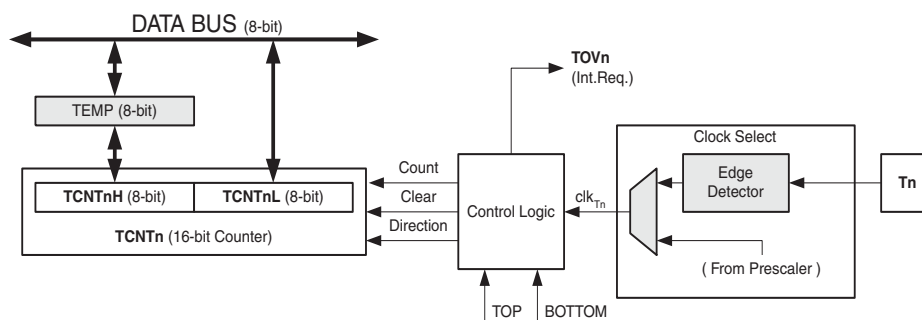
Figure 14-2. Counter Unit Block Diagram
