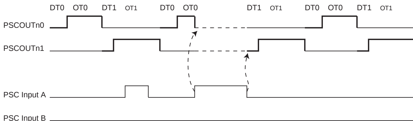
Figure 15-20. PSCn behaviour versus PSCn Input A in Fault Mode 1
