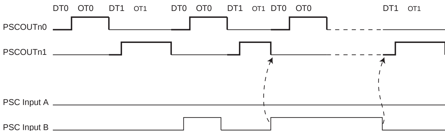
Figure 15-23. PSCn behaviour versus PSCn Input B in Fault Mode 2
