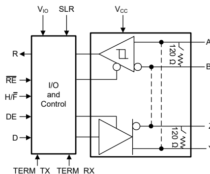
Simplified Schematic
