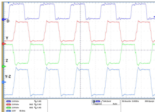
Figure 9-9. THVD1424 Driver Waveforms at 20 Mbps with Termination Enabled
