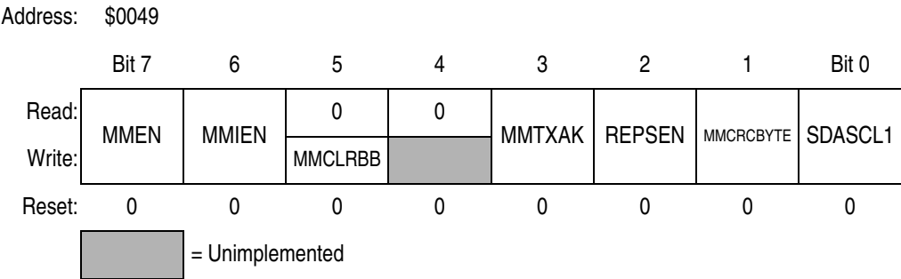
Figure 17-5. MMIIC Control Register 1 (MMCR1)
