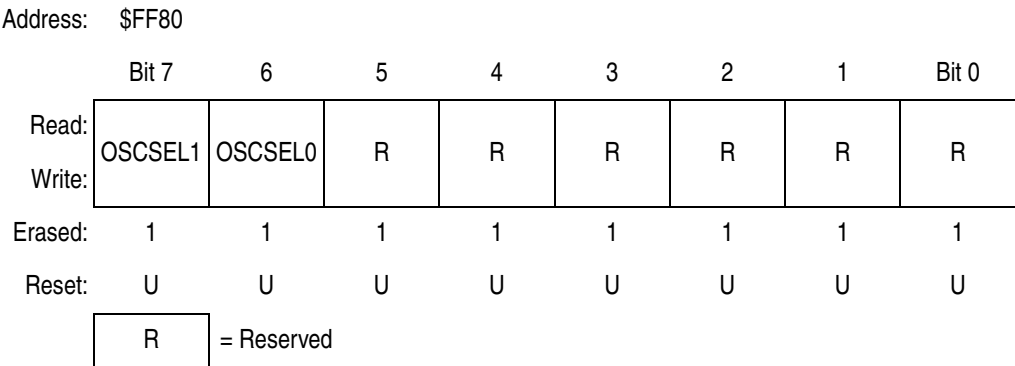
Figure 7-2. Mask Option Register (MOR)
