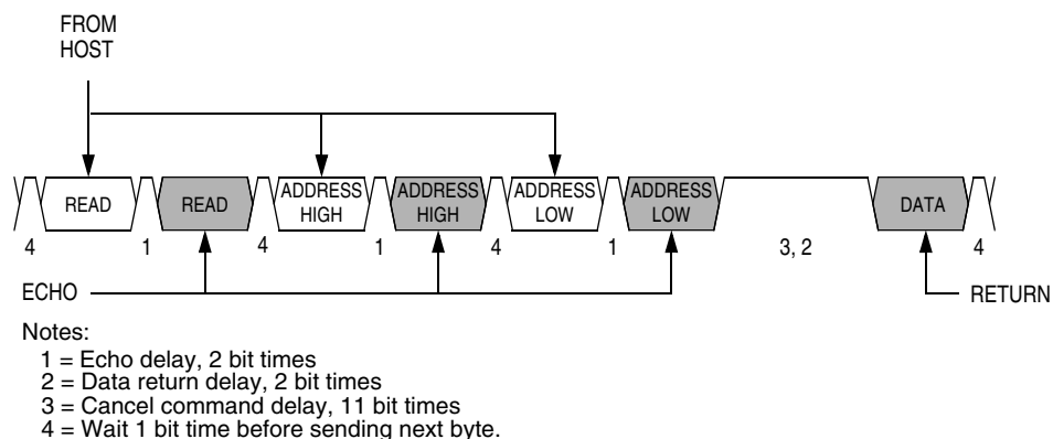
Figure 10-5. Read Transaction
