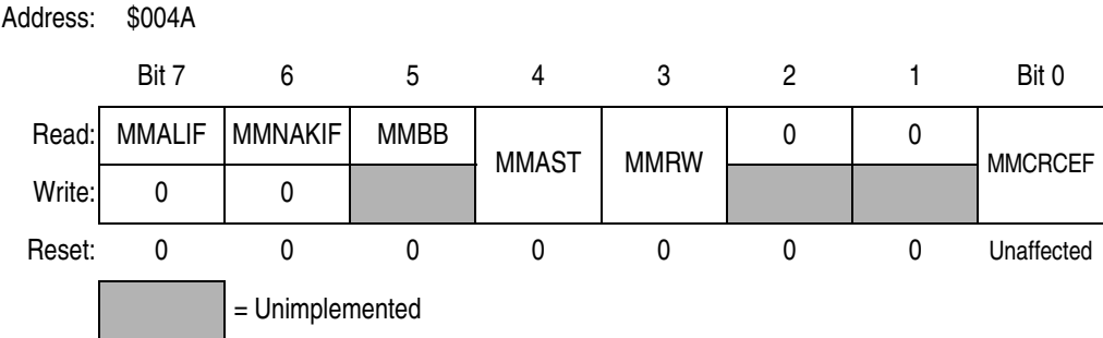
Figure 17-6. MMIIC Control Register 2 (MMCR2)
