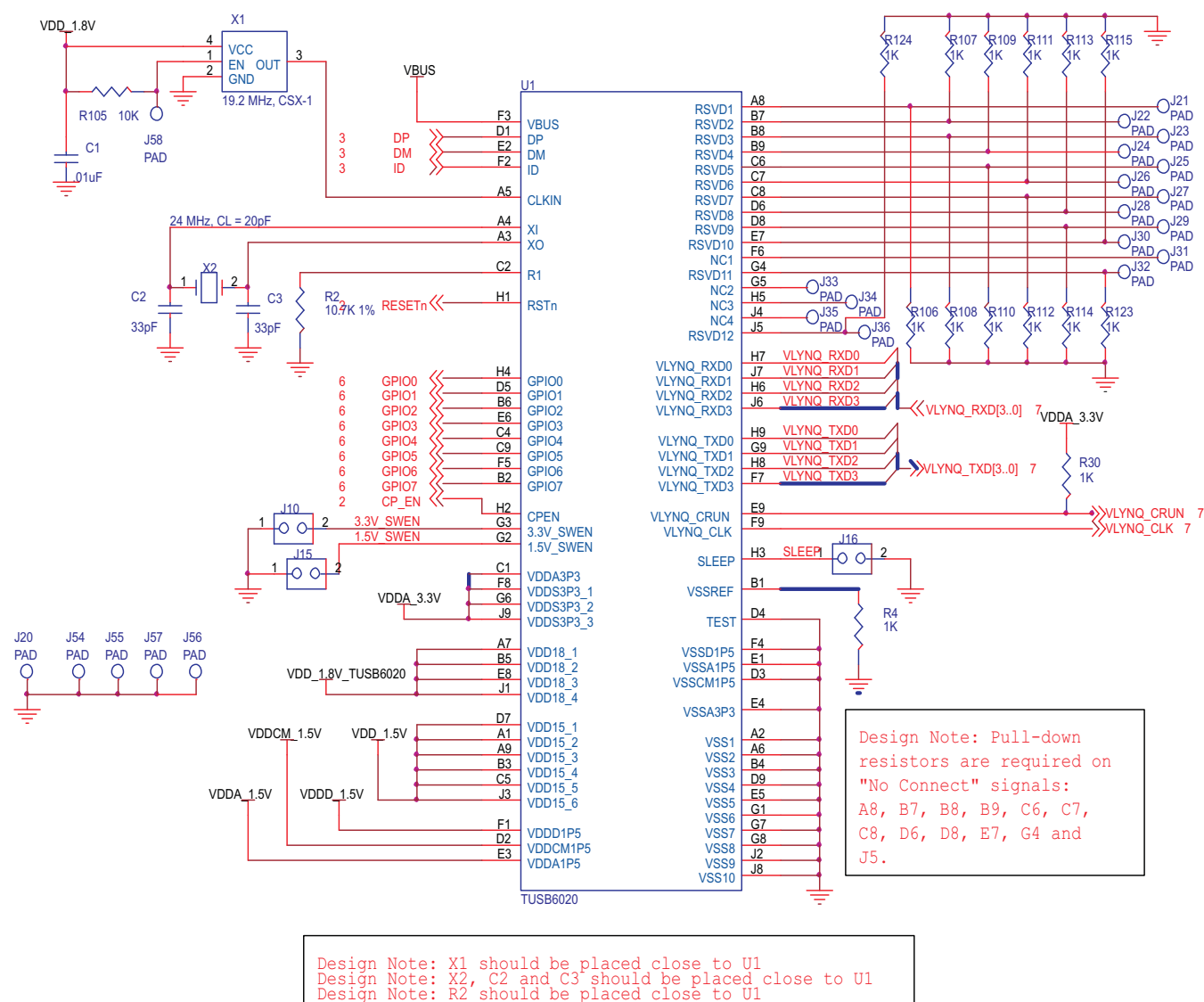
Figure 1-3. TUSB6020
