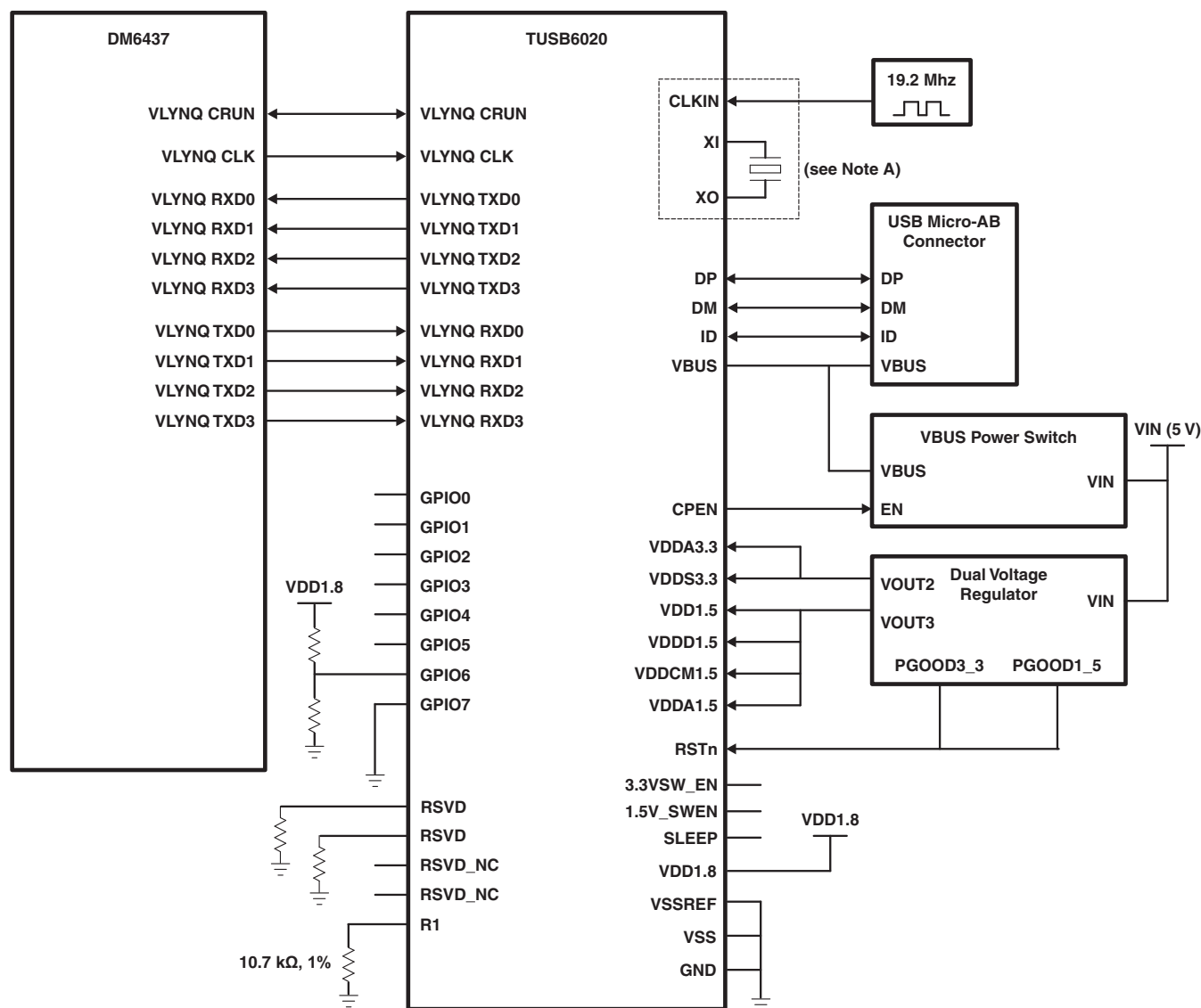
Figure 1-1. TUSB6020 Connection Block Diagram
