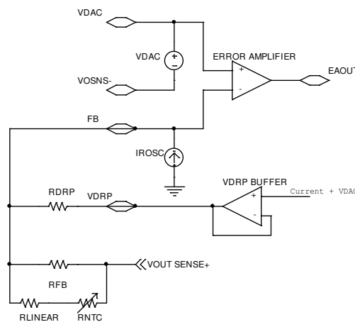
Figure 10- Temperature compensation of inductor DCR
